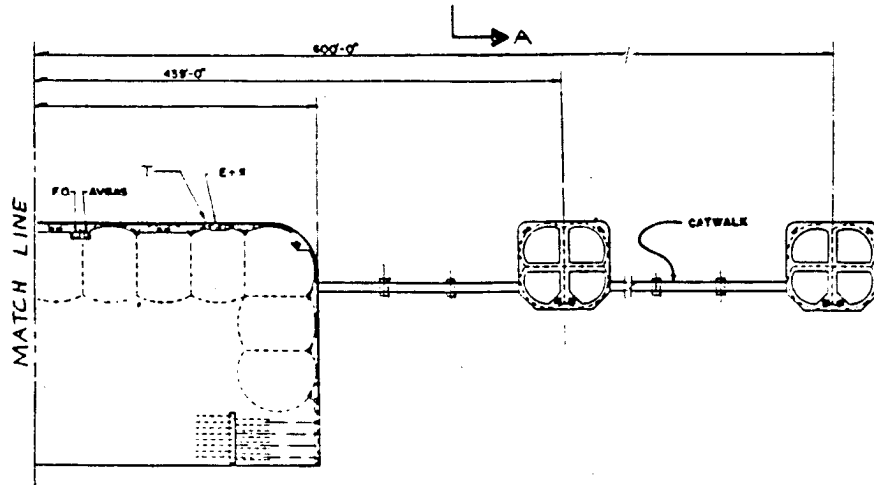
GENERAL PLAN
