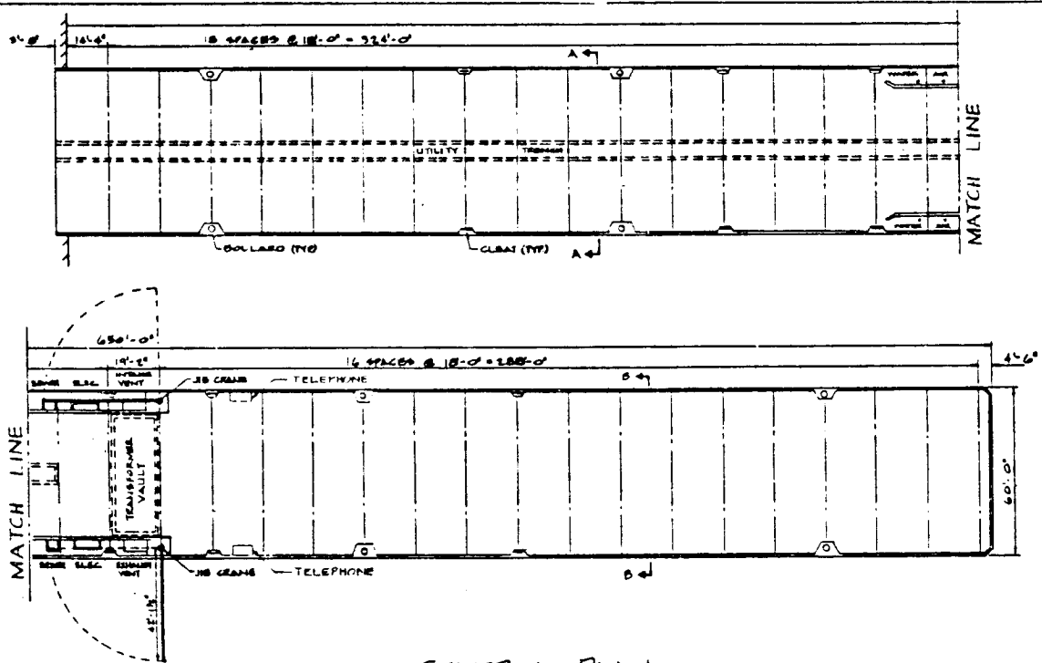
GENERAL PLAN
