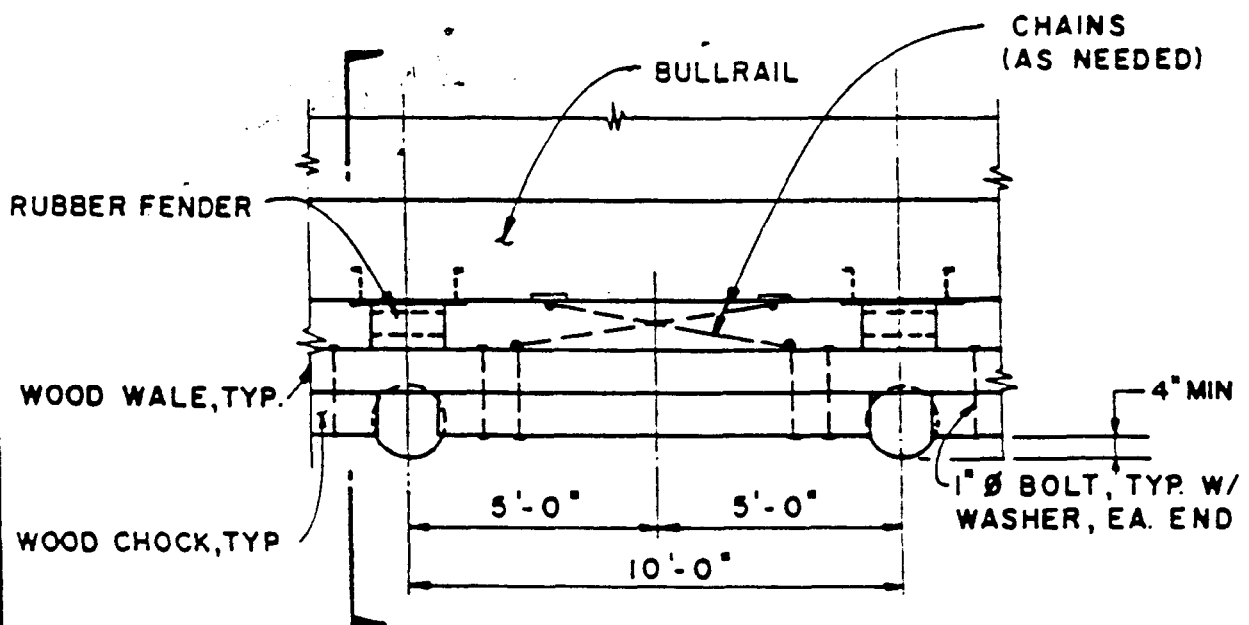
(A) PLAN OF FENDER SYSTEM
