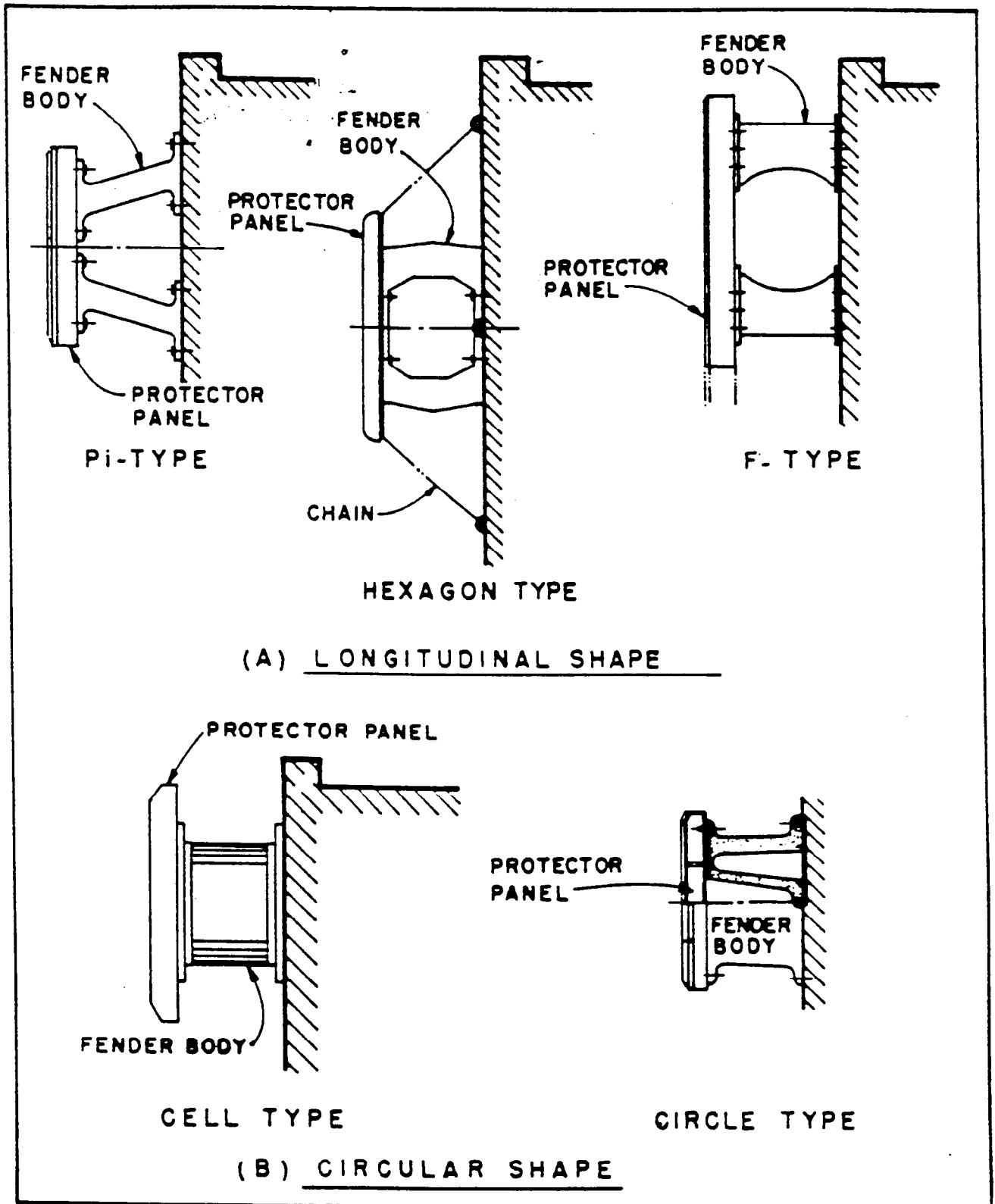
Figure 48 Buckling Fender with Contact Panel
