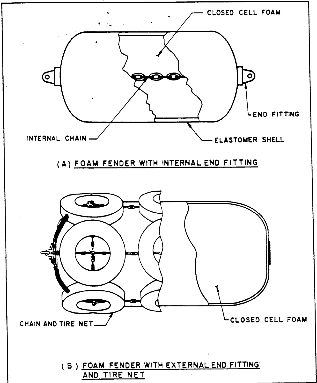
Figure 50 Foam-Filled Fenders
