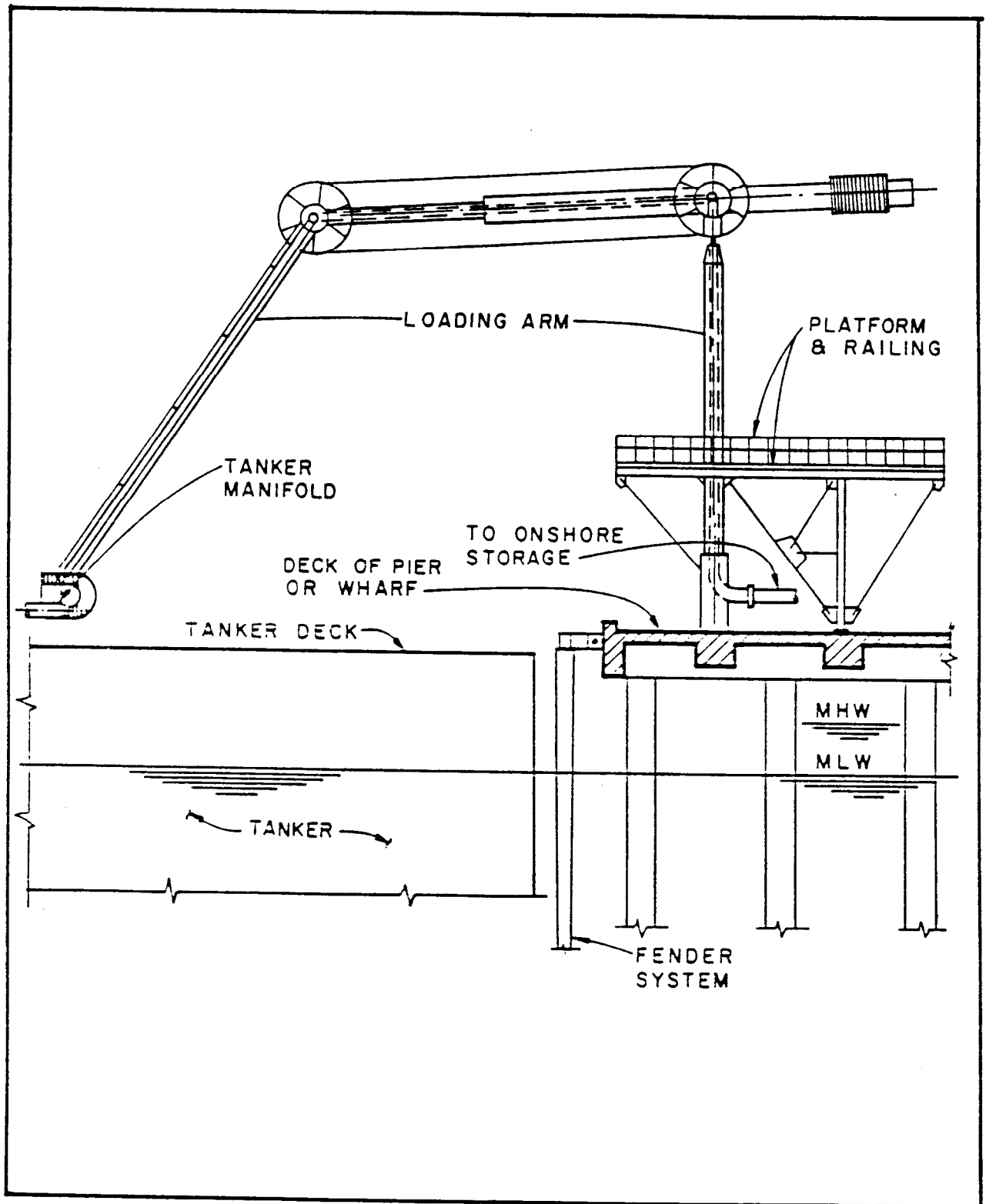
Figure 70 Fuel Loading Arm
