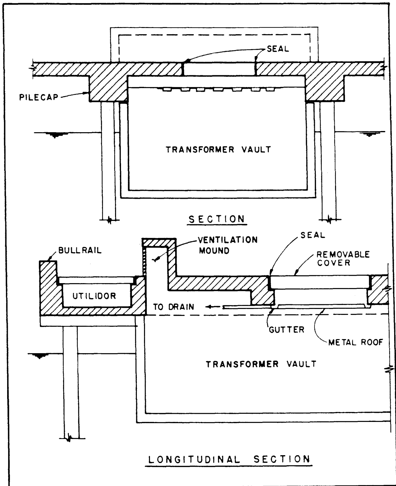
Figure 39 Transformer Vault
