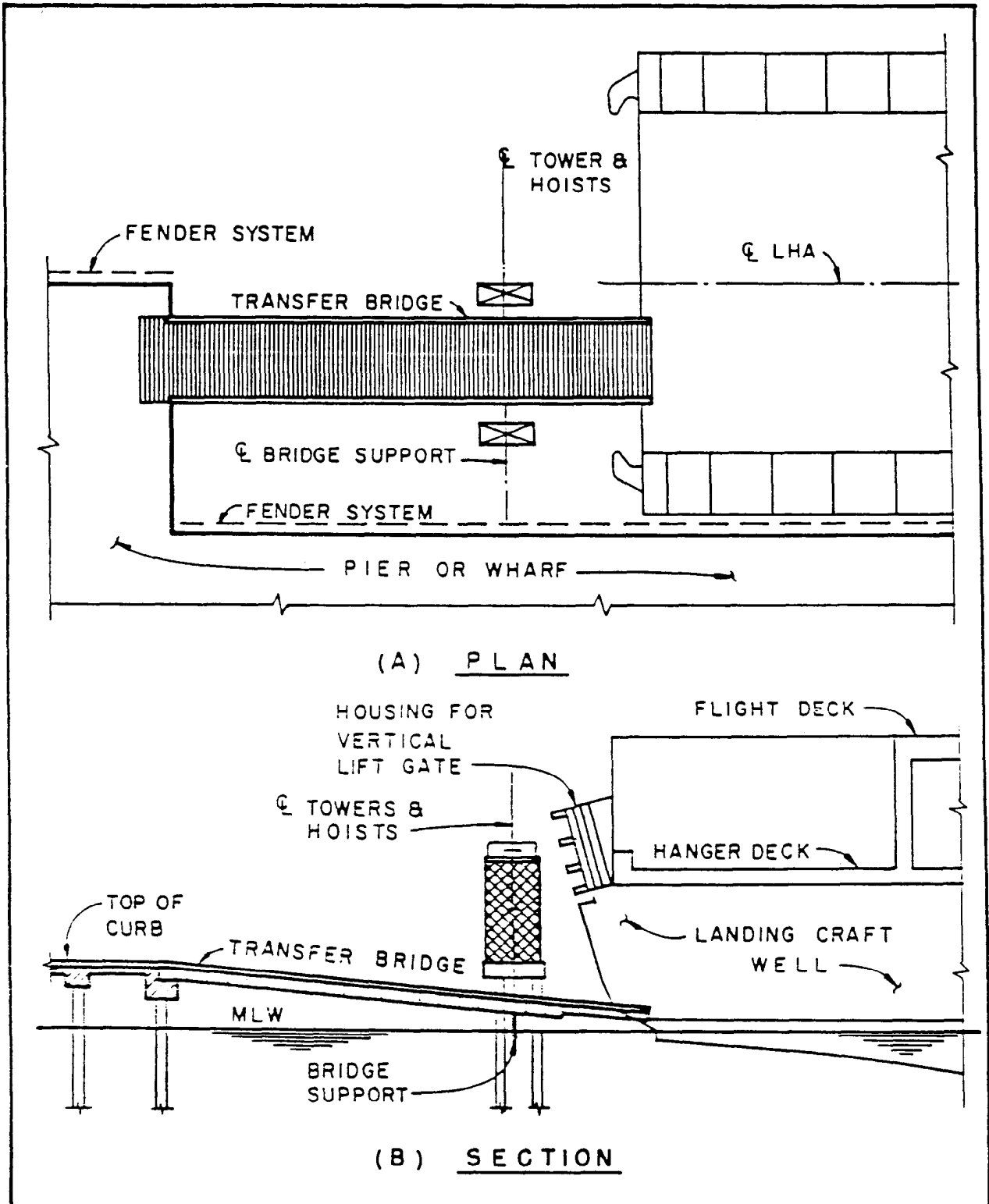
Figure 68 Transfer Bridge for LHAs
