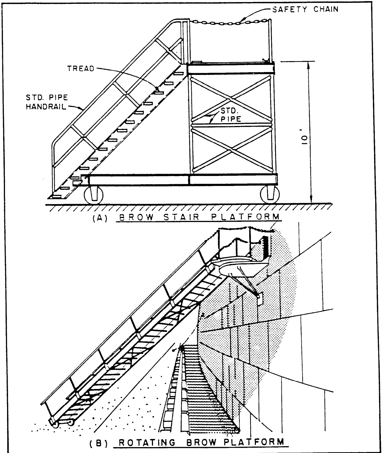
Figure 67 Brow Platforms
