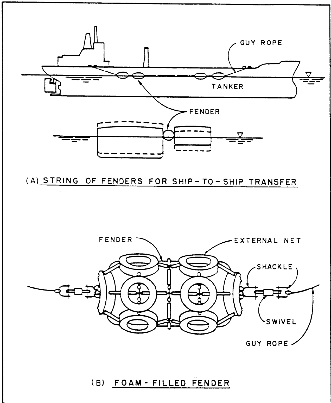
Figure 63 Foam-Filled Fender as Separator
