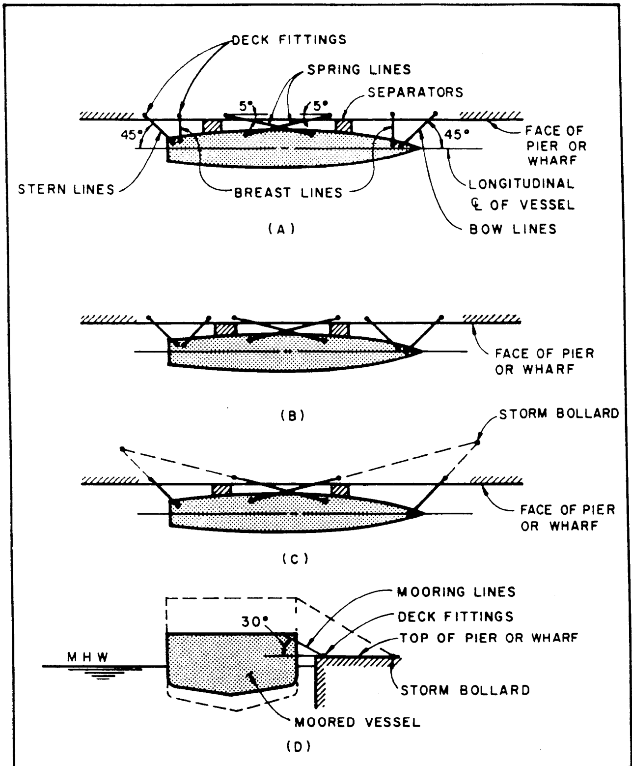
Figure 21 Mooring Arrangements
