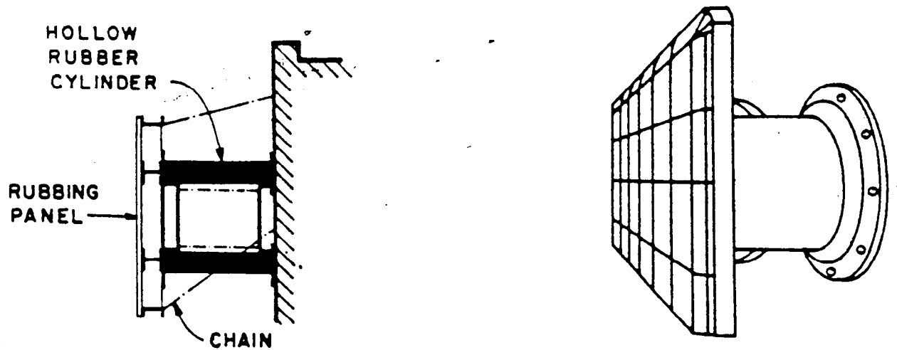
( A ) END-LOADED RUBBER FENDERS
