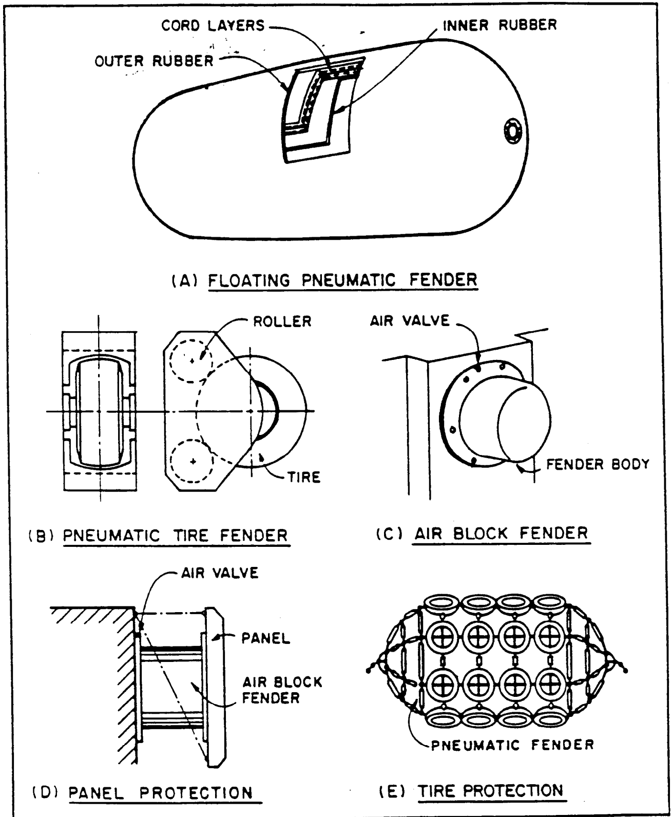
Figure 49 Pneumatic Fenders
