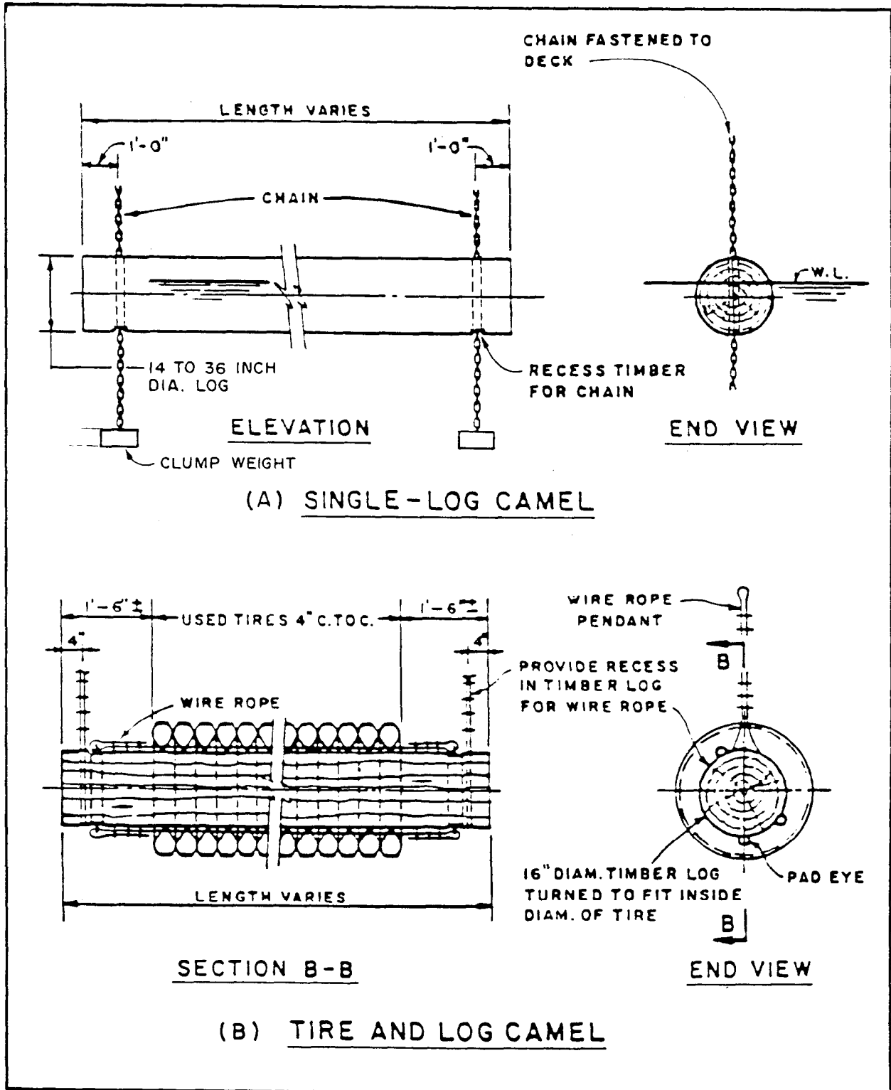
Figure 58 Log Camels
