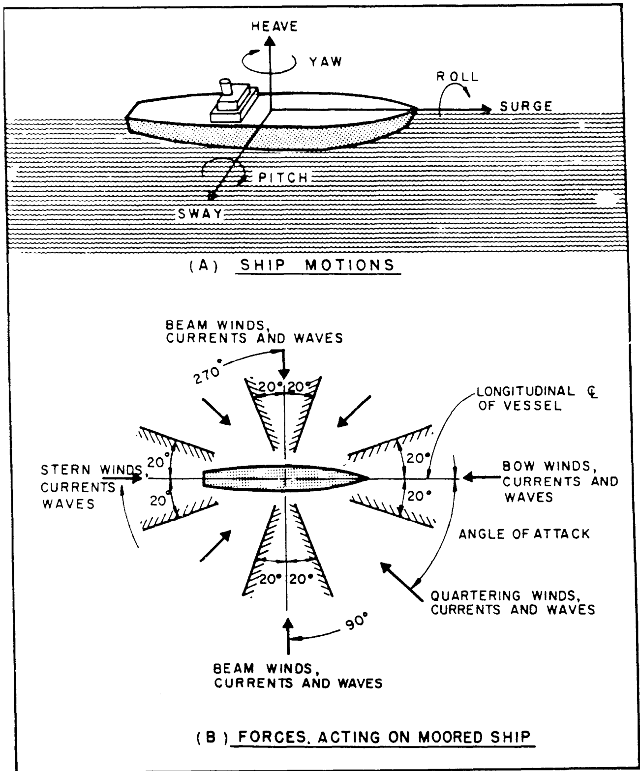
Figure 22 Ship Motions and Forces Acting on Ship
