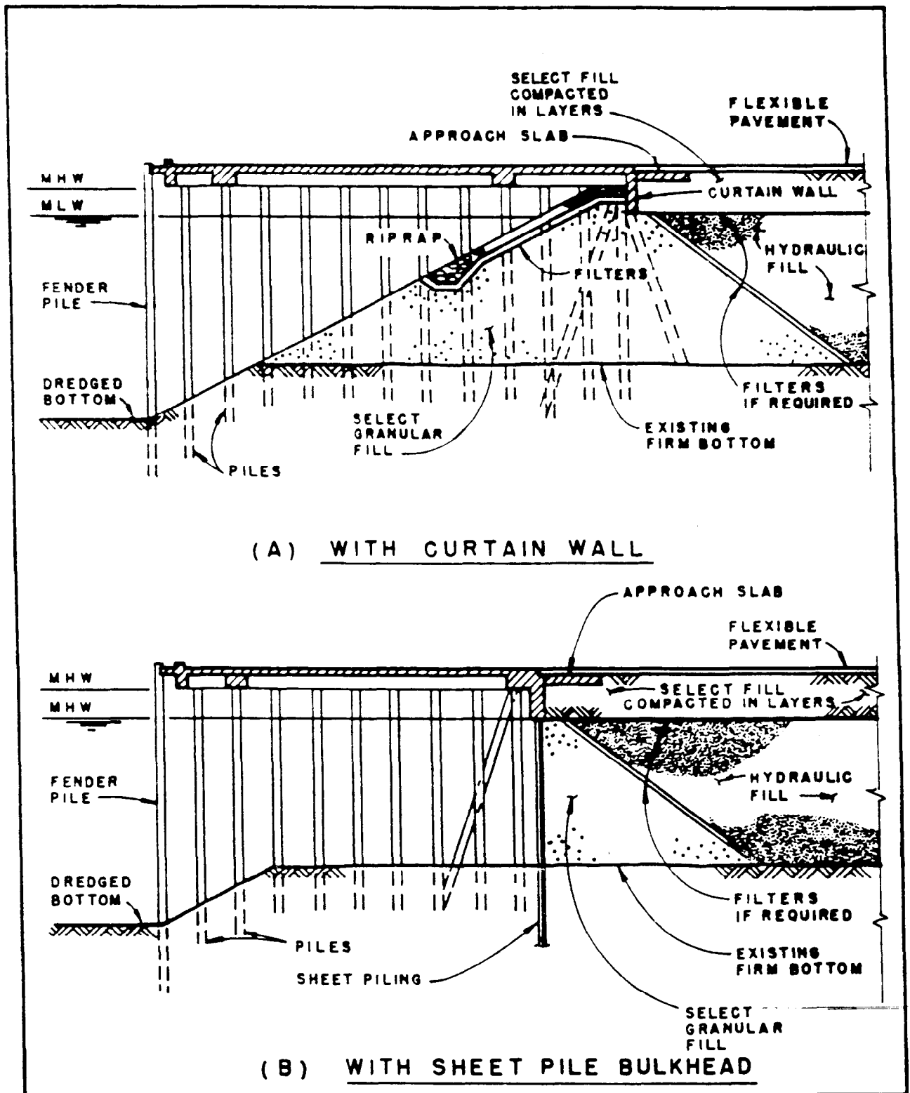
Figure 11 Open-Type Marginal Wharf Concepts
