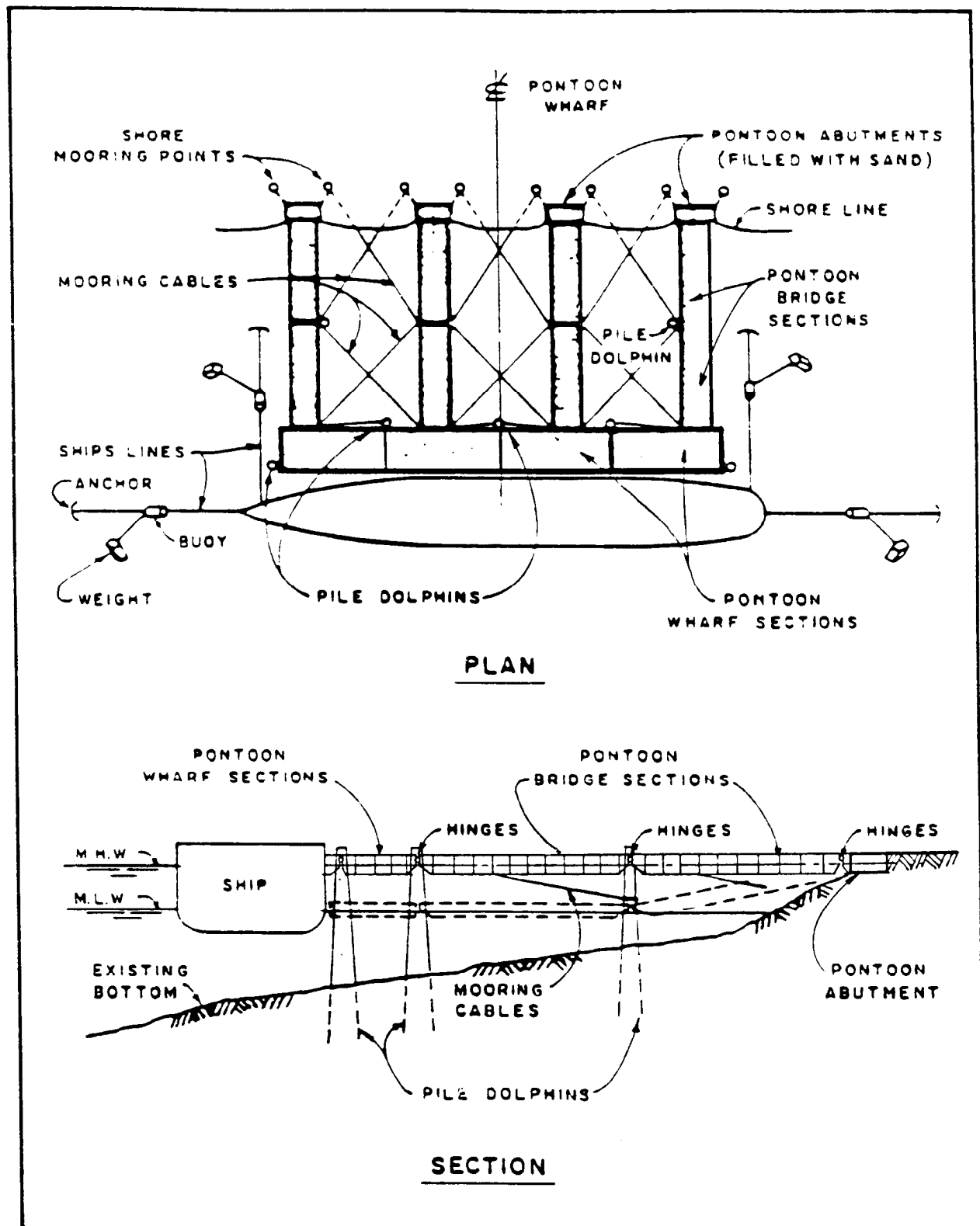
Figure 29 Pontoon Wharf
