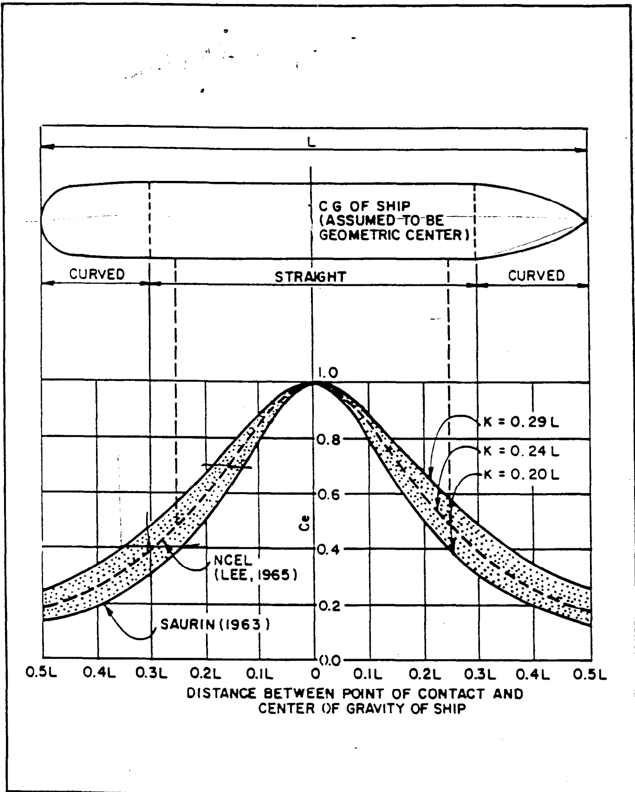
Figure 43 Eccentricity Coefficient, C
