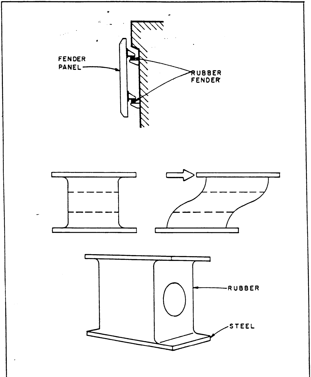
Figure 47 Shear Fender
