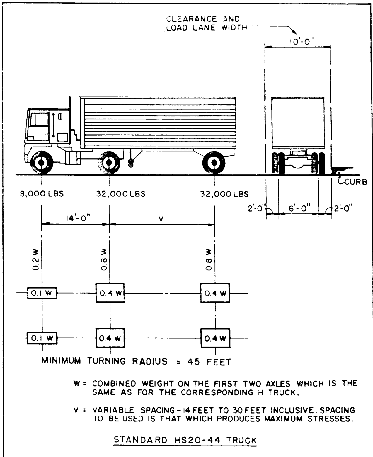
Figure 15 Truck Loading
