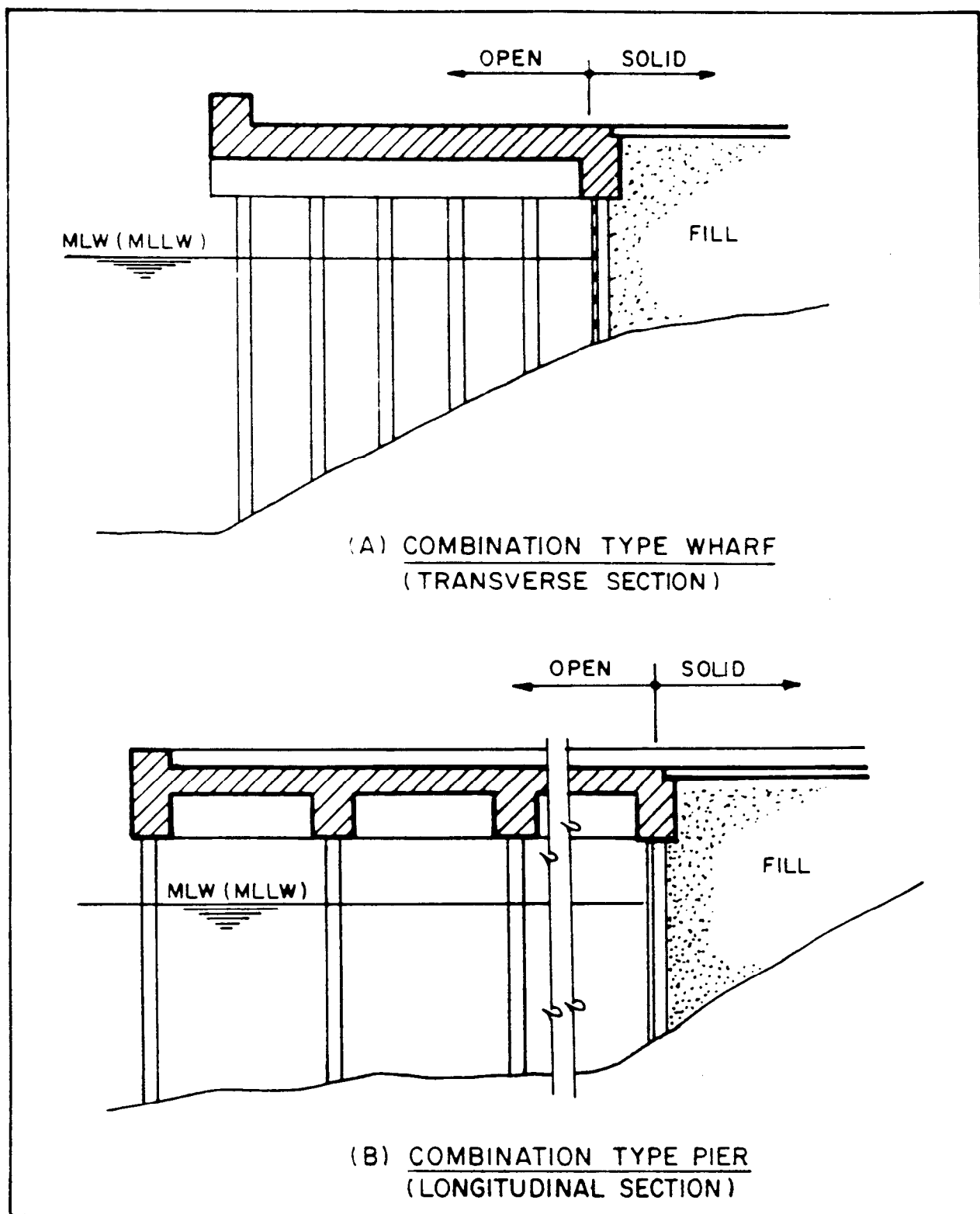
Figure 10 Combination Types
