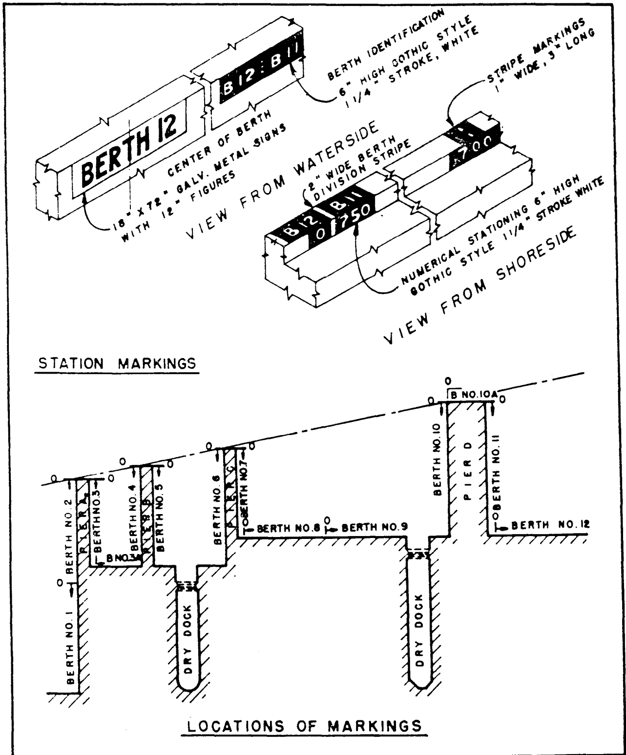
Figure 41 Layout of Berth and Station Markings
