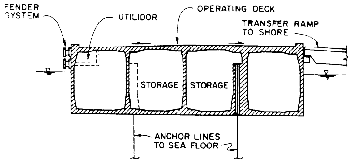
(A) FLOATING PONTOON TYPE (WHARF)
