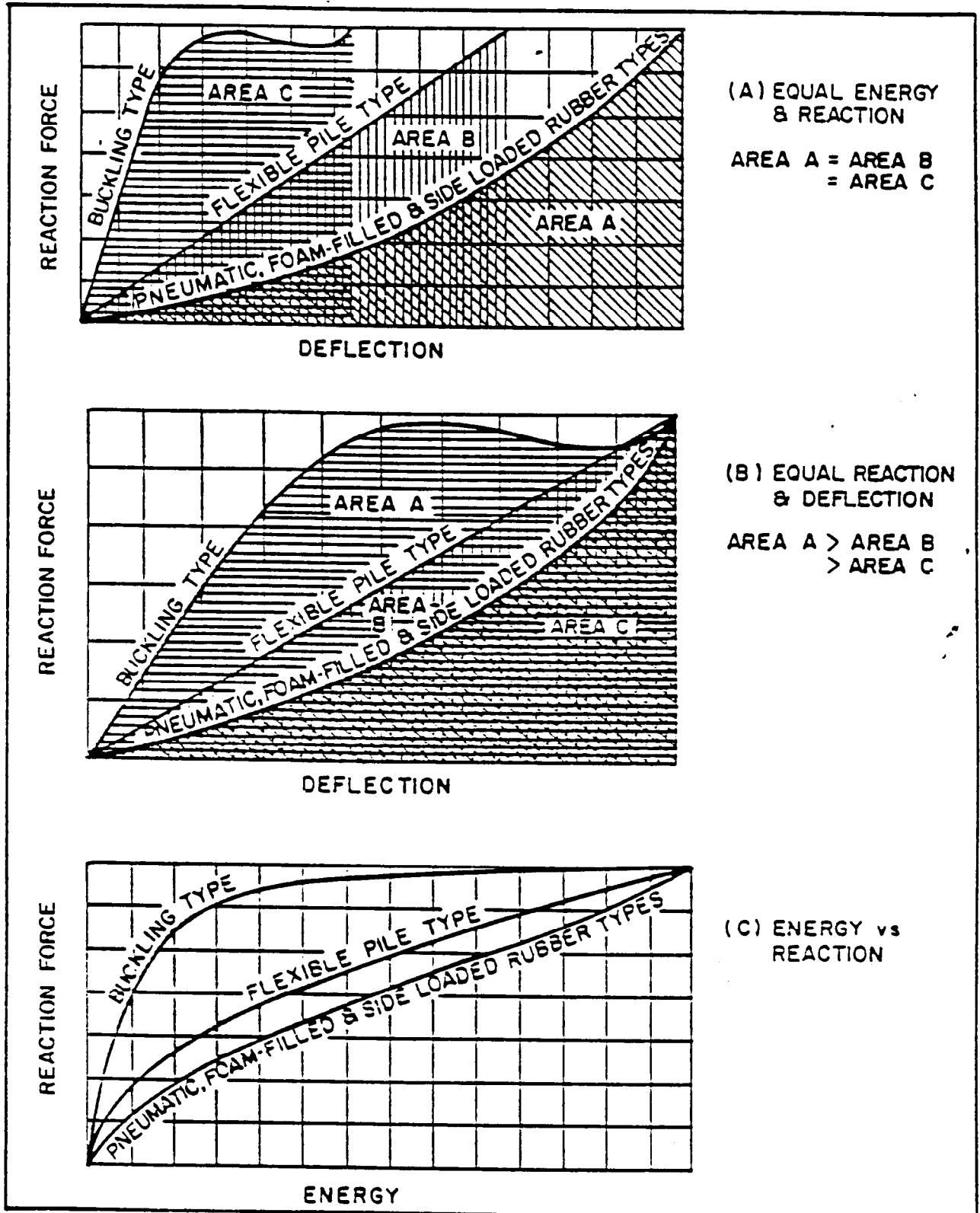
Figure 56 Evaluation of Fender System Types
