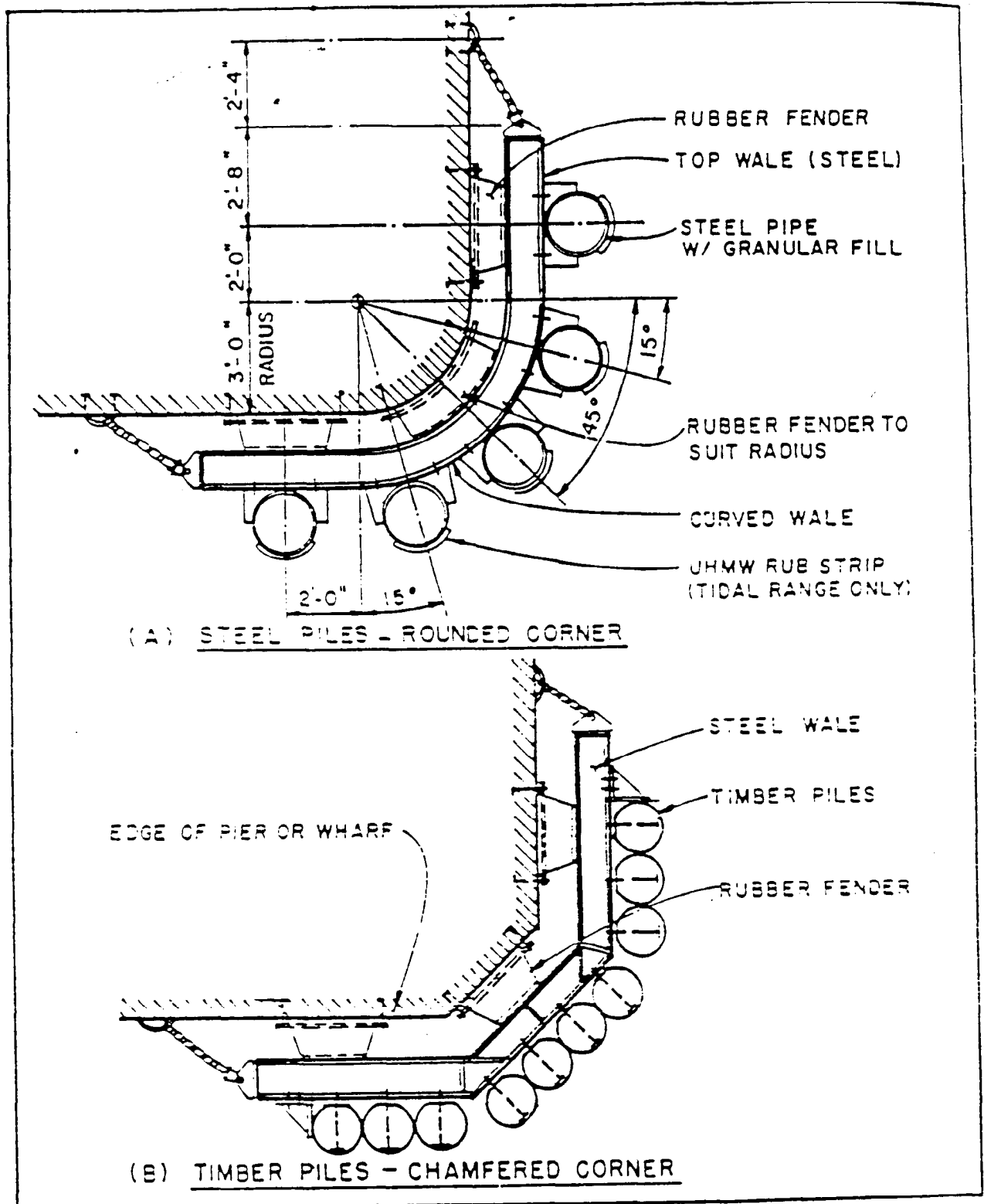
Figure 57 Corner Protection 134
