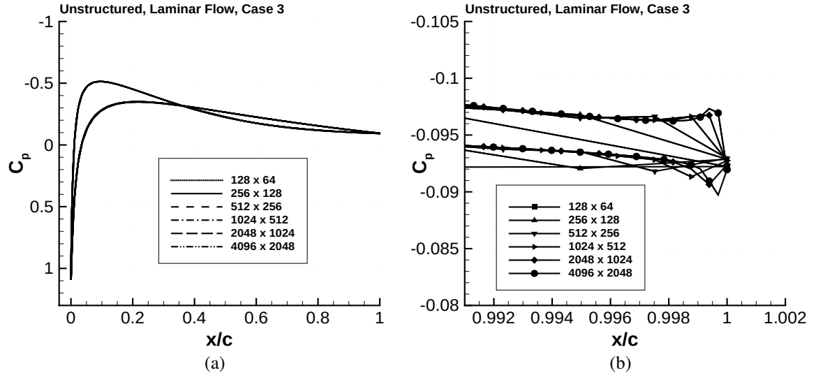
Figure 28: Surface pressure distributions for Case 3 computed with unstructured grid method. (a) Surface pressures, (b) Trailing edge region.
