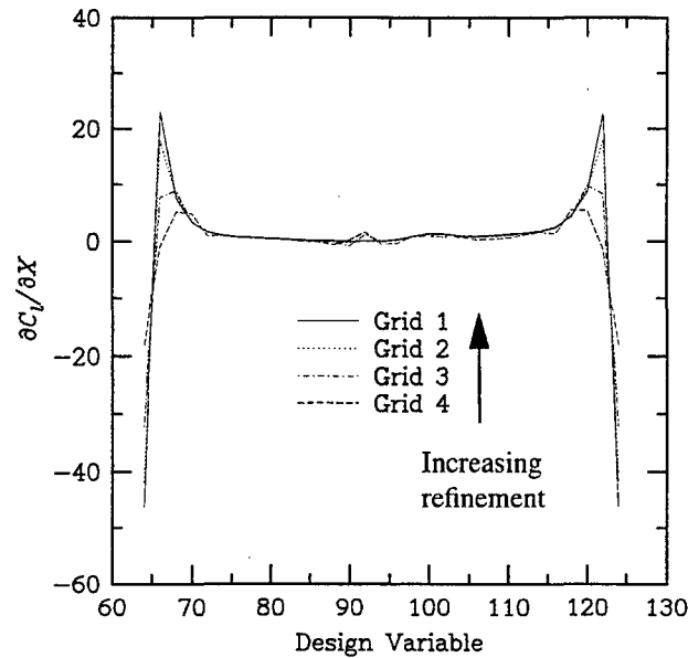
Figure 13. Sensitivity derivatives.
