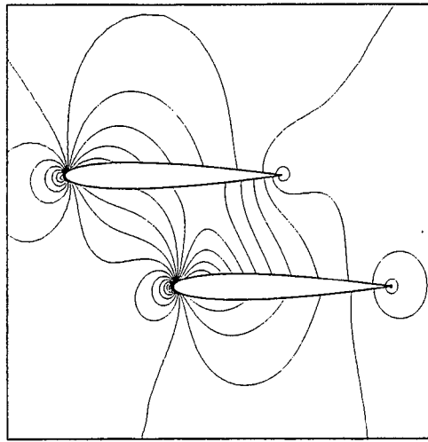
Figure 20. Final airfoils and pressure coefficient for two-element airfoil.
