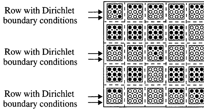
Figure 4. Matrix structure for continuous adjoint approach.
