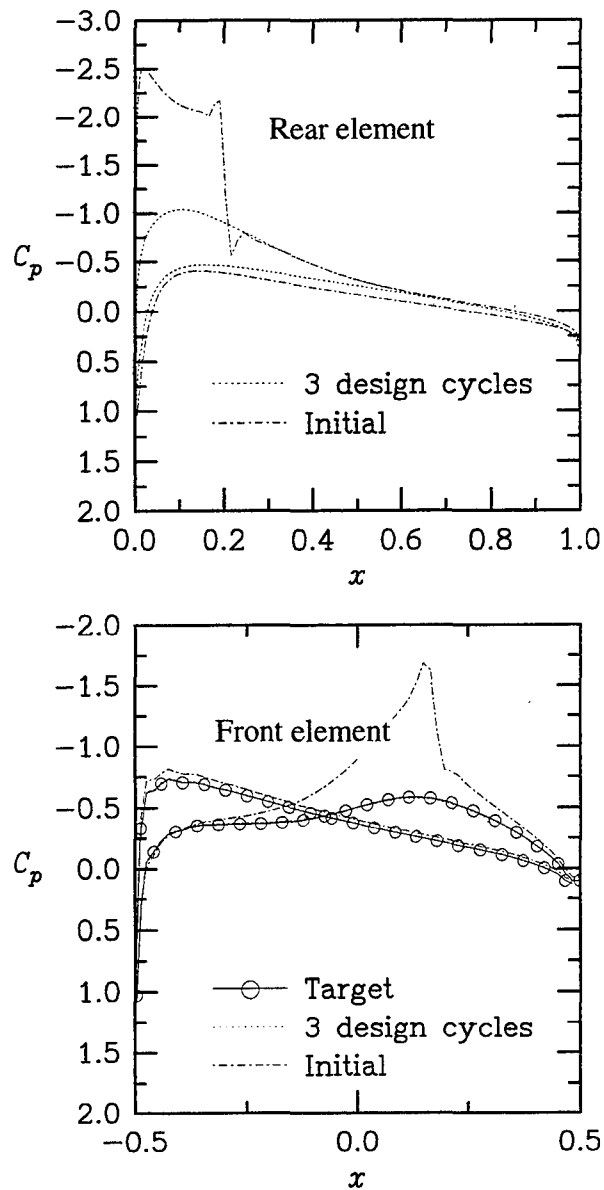
Figure 19. Initial and final pressure distributions for two-element test case.
