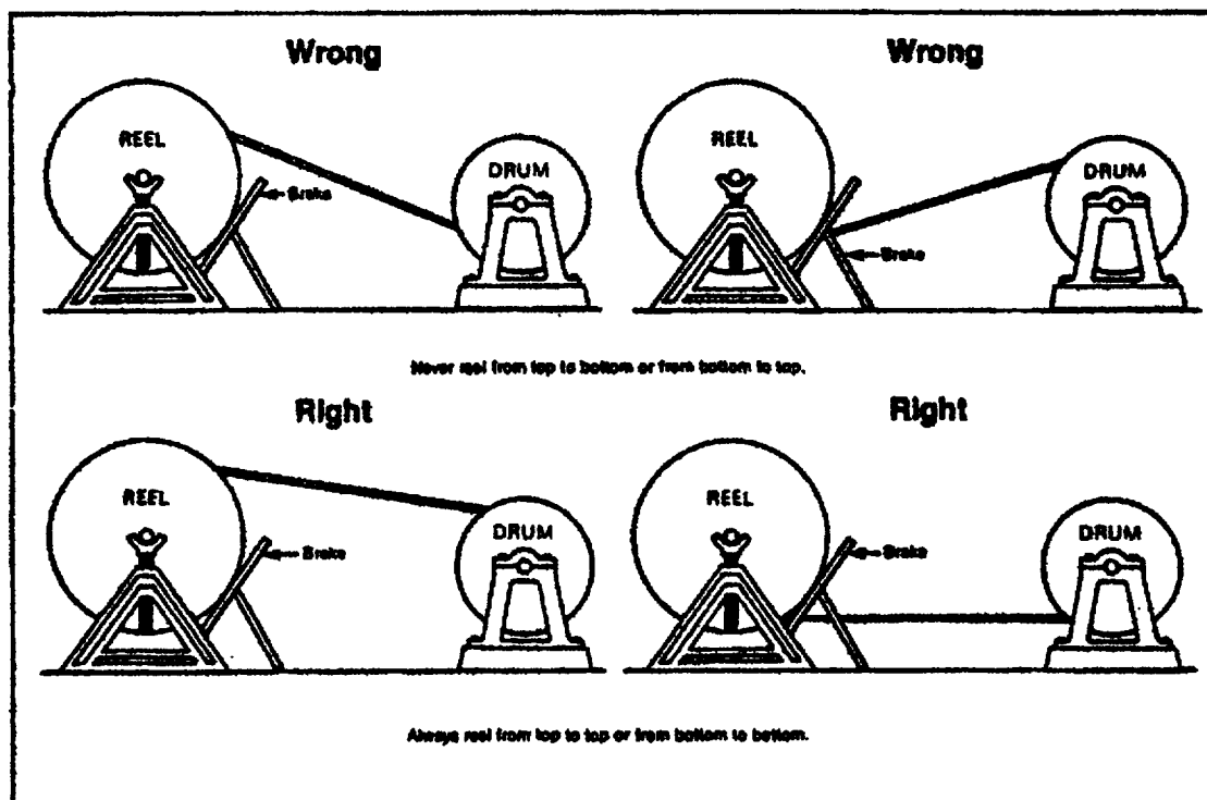
Fig. 2-11 Methods of winging rope from reel to drum, or reel to reel Rigging Manual, D.E. Dickie, P.ENG. Construction Safety Association of Ontario, Oct. 1975
