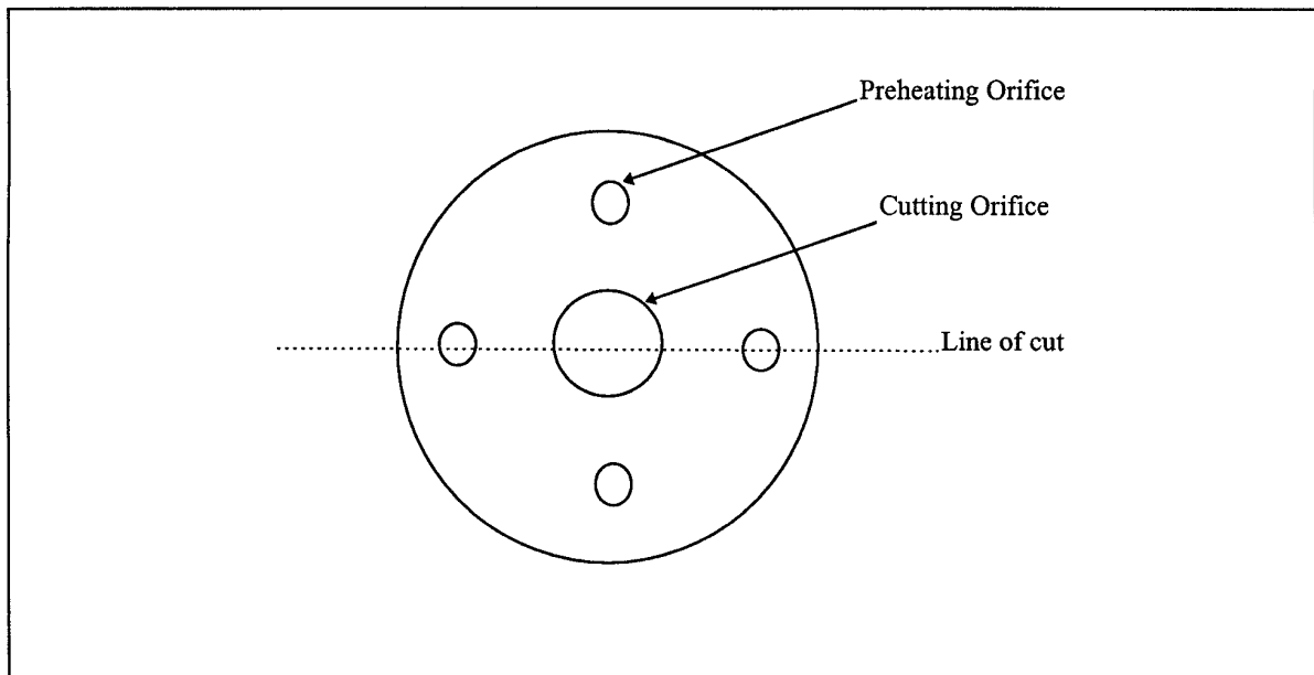
Fig. 3-10 Cutting tip cross section.
