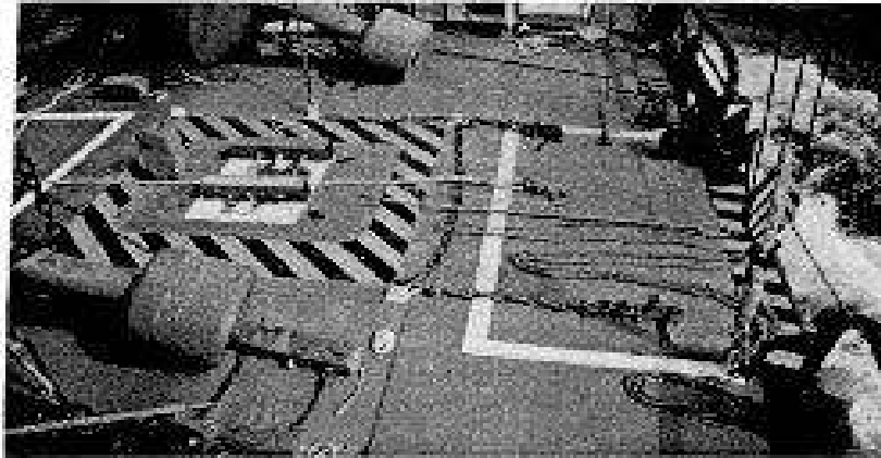
Fig. 8-1 Buoy deck layout when approaching a buoy
