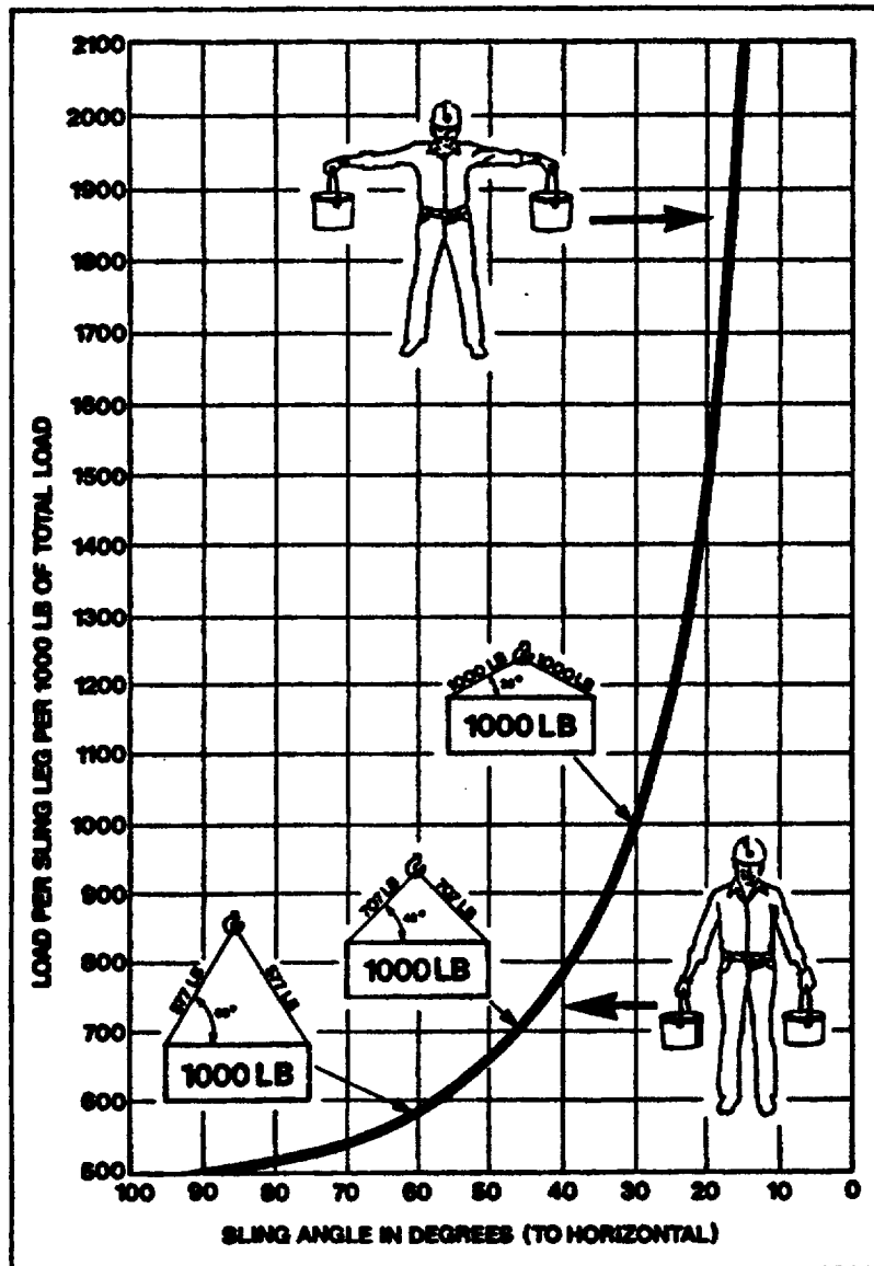
Fig. 2-4 Load increases rapidly as the angle of the sling over the load decreases
