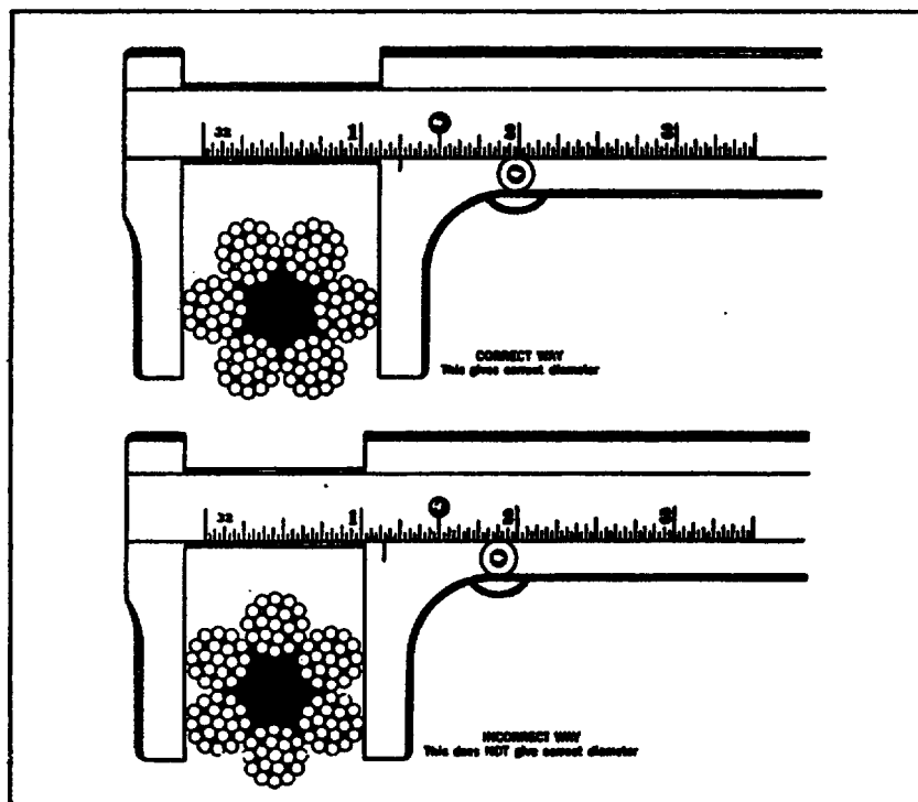
Fig. 2-8 Measuring wire rope diameter Rigging Manual, D.E. Dickie, P.ENG. Construction Safety Association of Ontario, Oct. 1975
