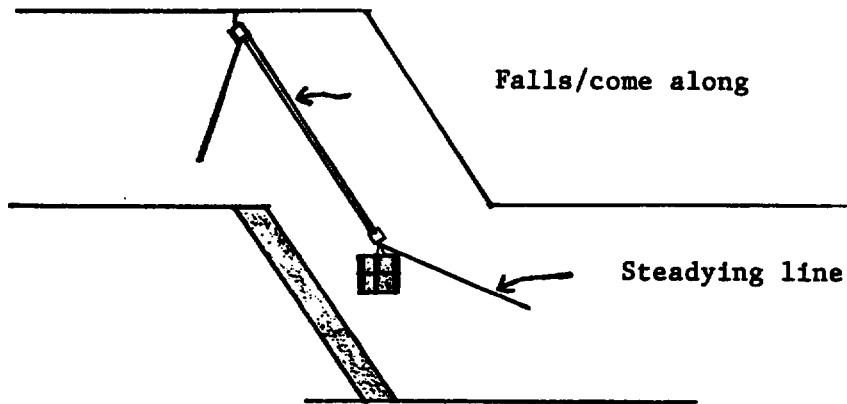
Fig. 7-3 Moving draft up/down ladder
