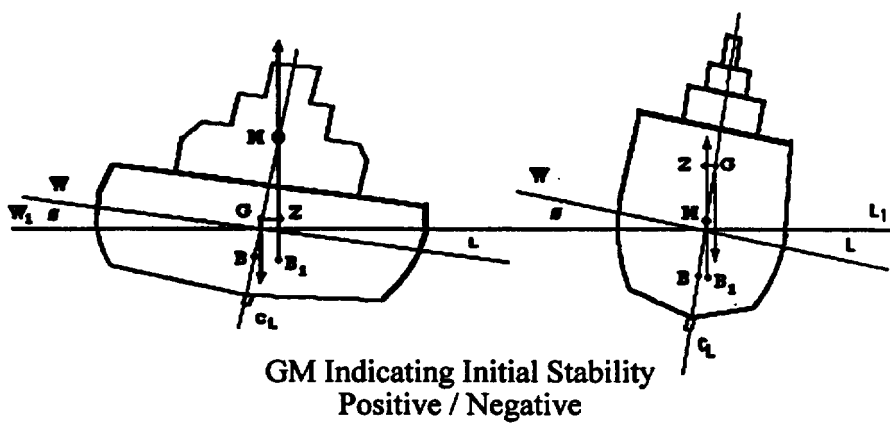
Fig. 7-6a Vessel in stable condition
