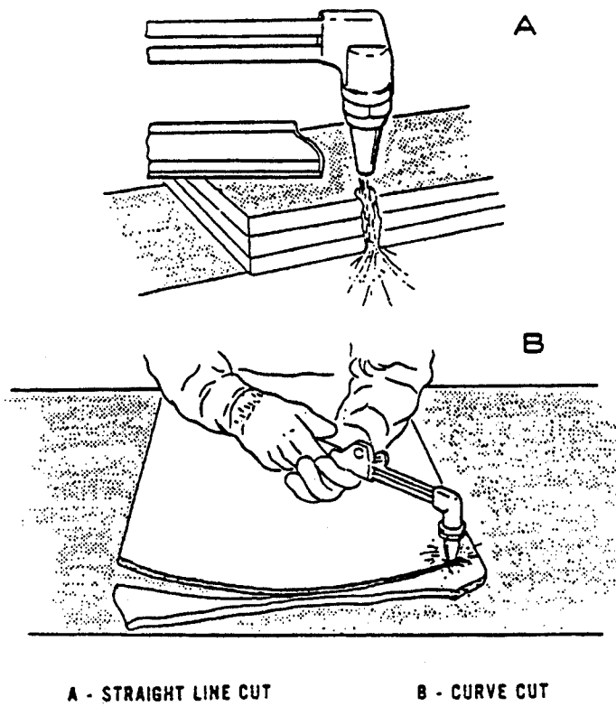
Figure 3-13 Cutting with a torch
