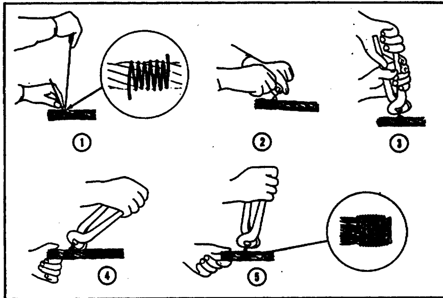
Fig. 2-14 Applying wire rope seizing
