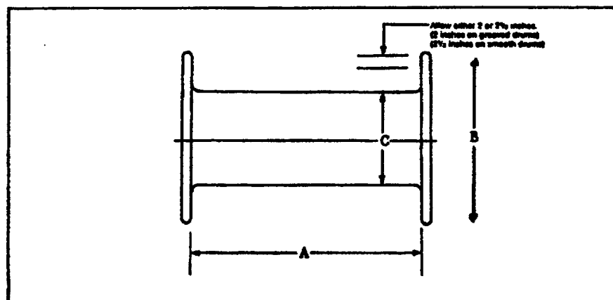
Fig. 2-12 Computing length of wire rope on reel
