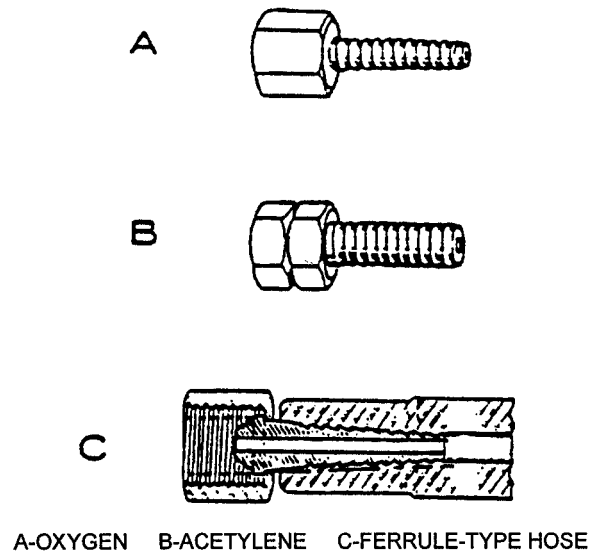
Figure 3-6 Hose Connections
