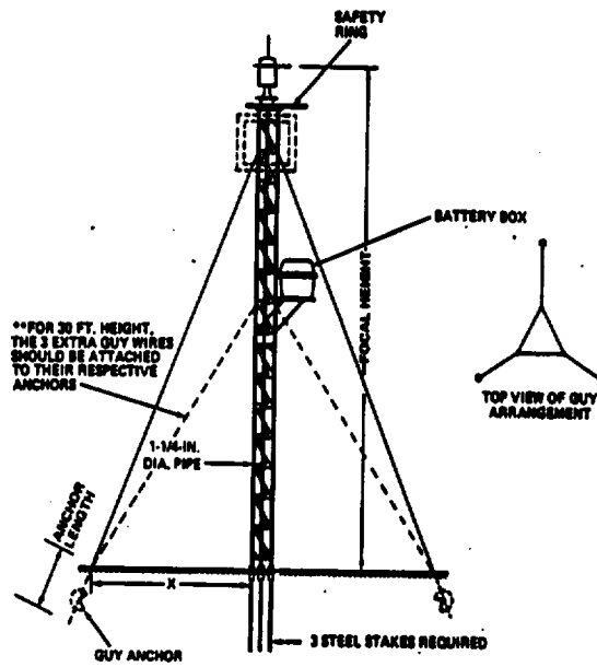
Figure 4-21. Single guyed skeleton tower. Data Sheet 4-0(9). (cont'd).
