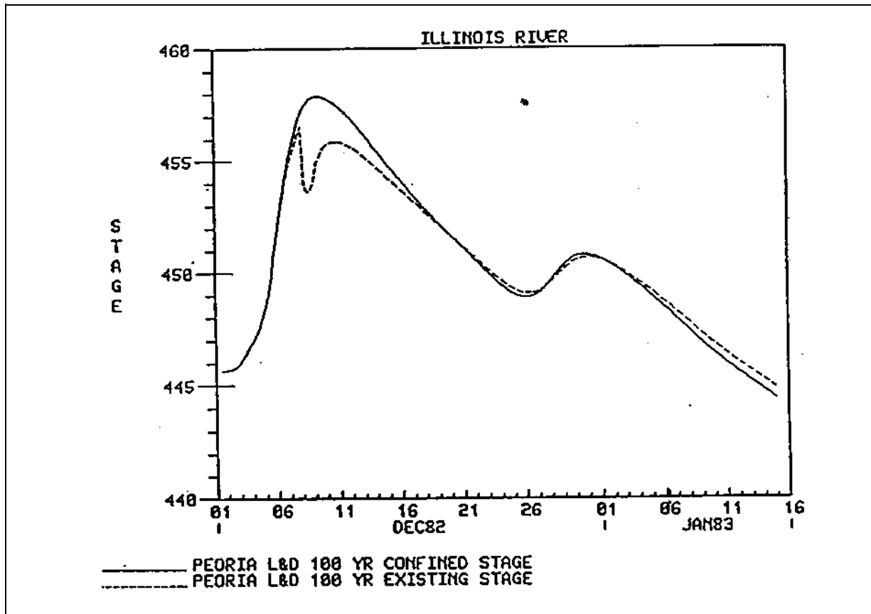
Figure D-9. Stage hydrographs for the Illinois River at Peoria with and without failures
