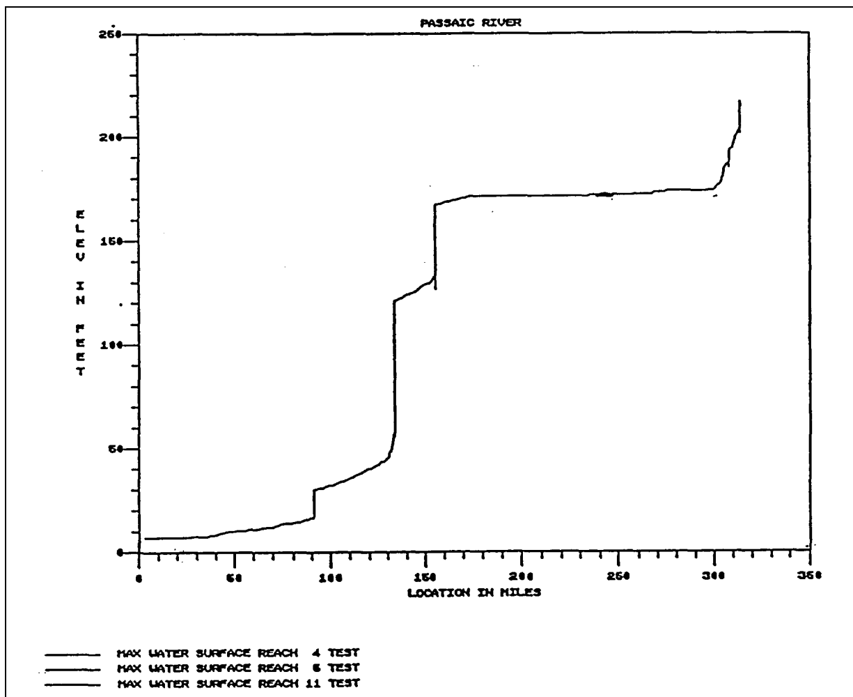
Figure D-7. The maximum water surface for a synthetic event on the Passaic River in New Jersey
