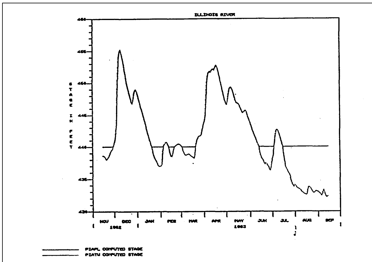
Figure D-5. Peoria Lock and Dam pool and tailwater hydrographs
