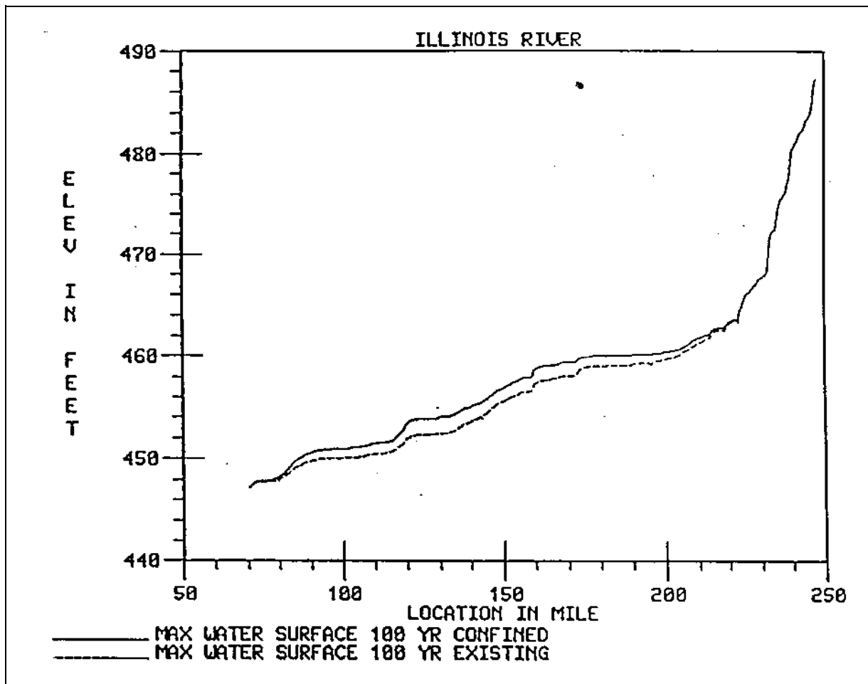
Figure D-10. The 100-yr maximum water surface along the Illinois River with and without levee failure
