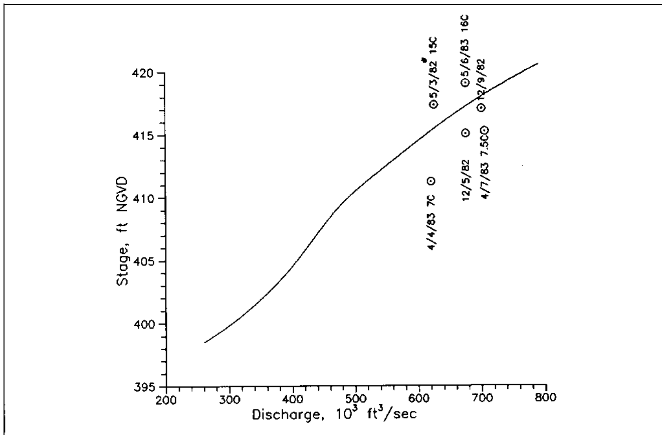
Figure D-18. Discharge measurements during the Dec. 1982, April and May 1983 floods at St. Louis, plotted with the St. Louis rating curve (Water temperature also shown in °C.)
