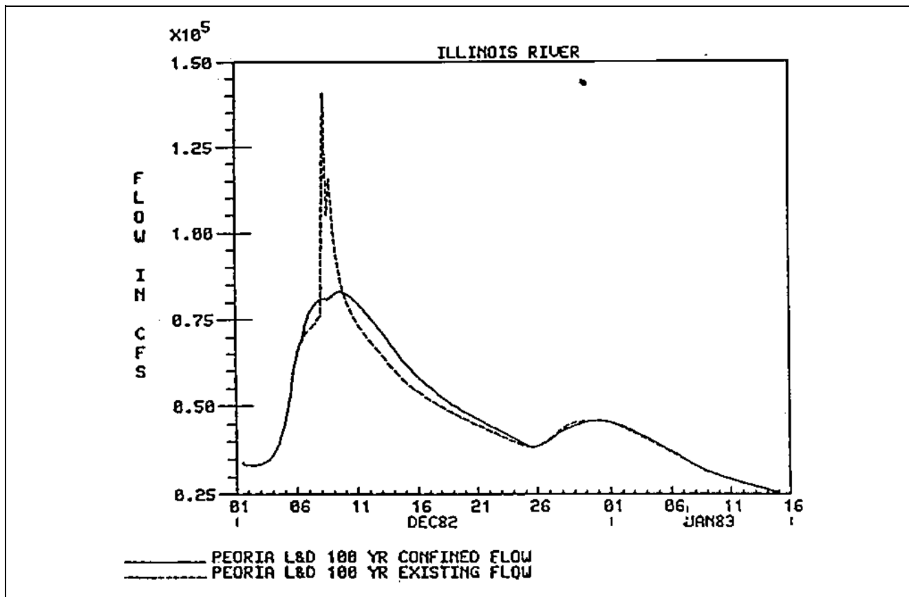
Figure D-12. Flow hydrographs for the Illinois River at Peoria with and without levee failure
