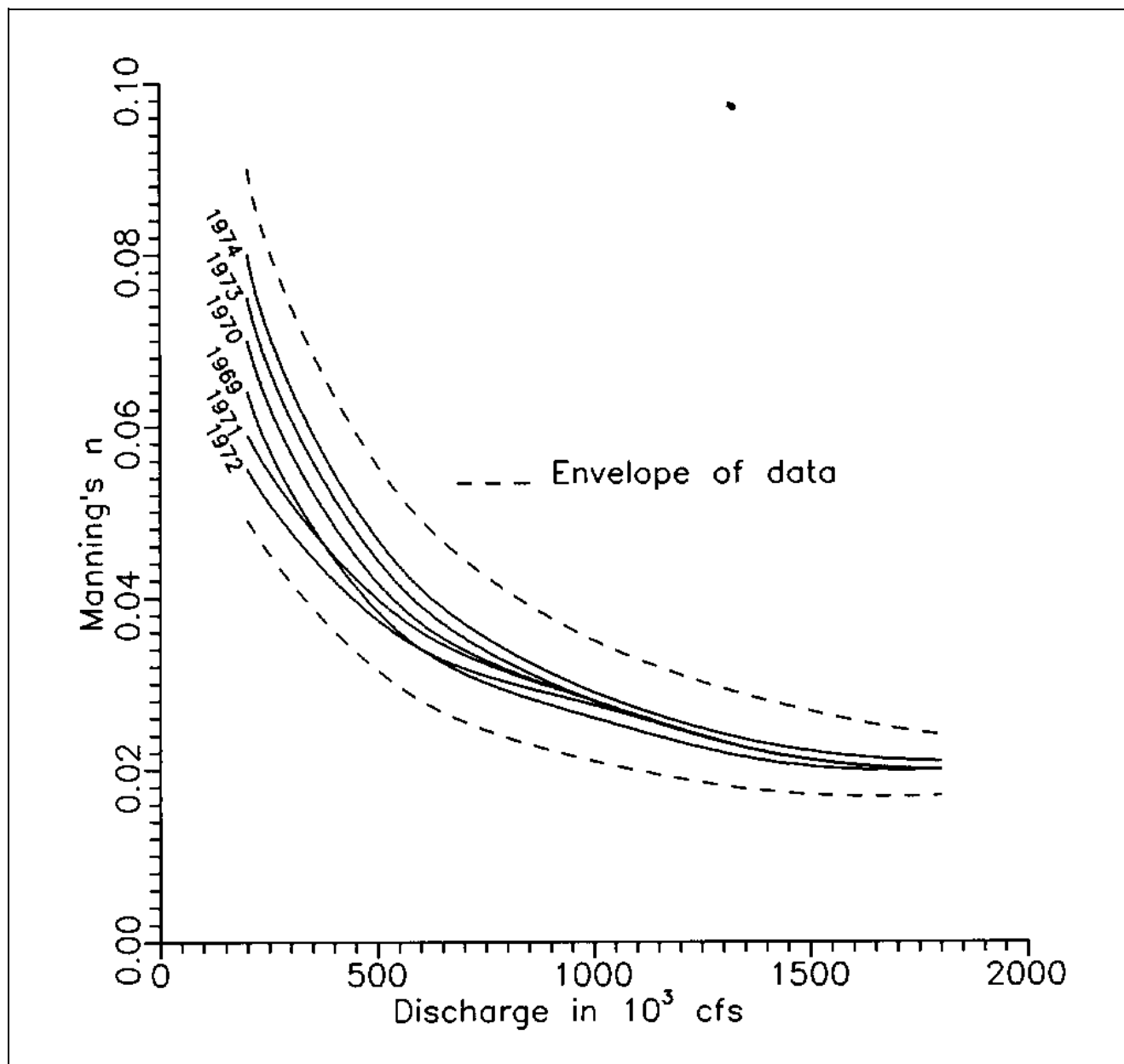
Figure D-14. Variation of Manning's n with discharge for the Mississippi River at Arkansas City (Source: St. Louis District, U.S. Army Corps of Engineers)
