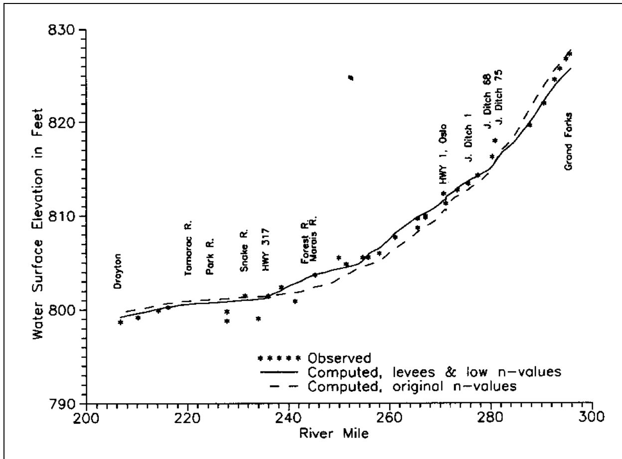
Figure 3-3. Profile calibration to high water marks
