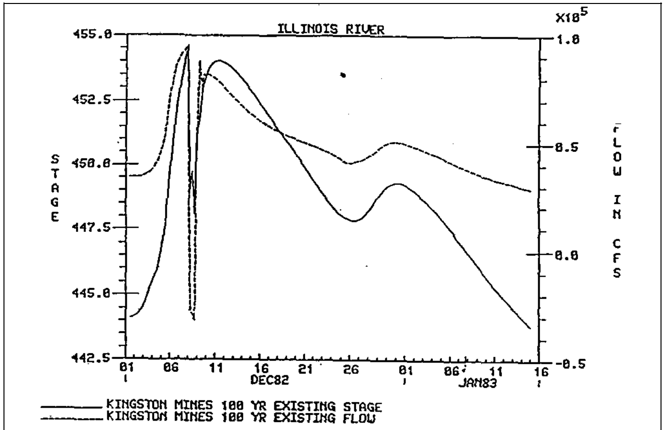
Figure D-13. Flow hydrographs for the Illinois River at Kingston Mines
