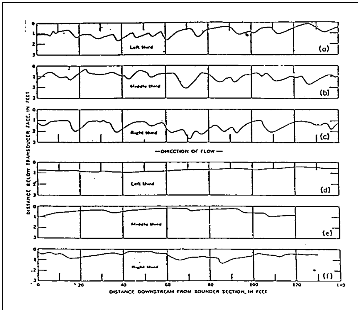
Figure D-16. Two sets of three longitudinal bed profiles each of Middle Loup River at Dunning, Neb., at high and low water temperature (Colby and Scott 1965)
