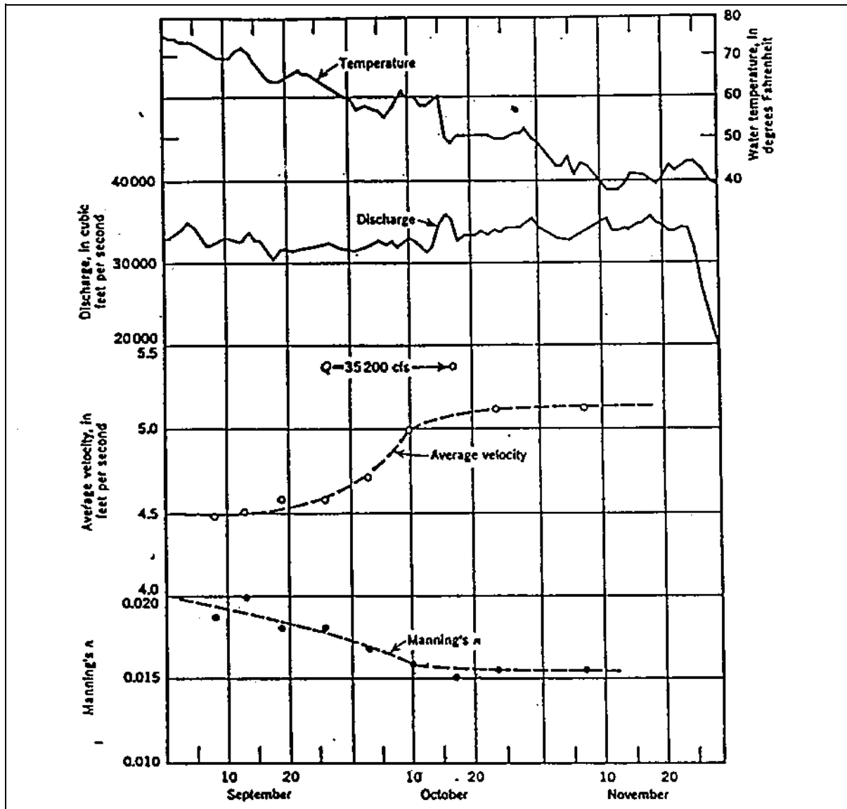
Figure D-17. Variation of water temperature, discharge, average velocity, and Manning's n for Missouri River at Omaha, Neb., during fall of 1966 (U.S. Army Corps of Engineers 1969)
