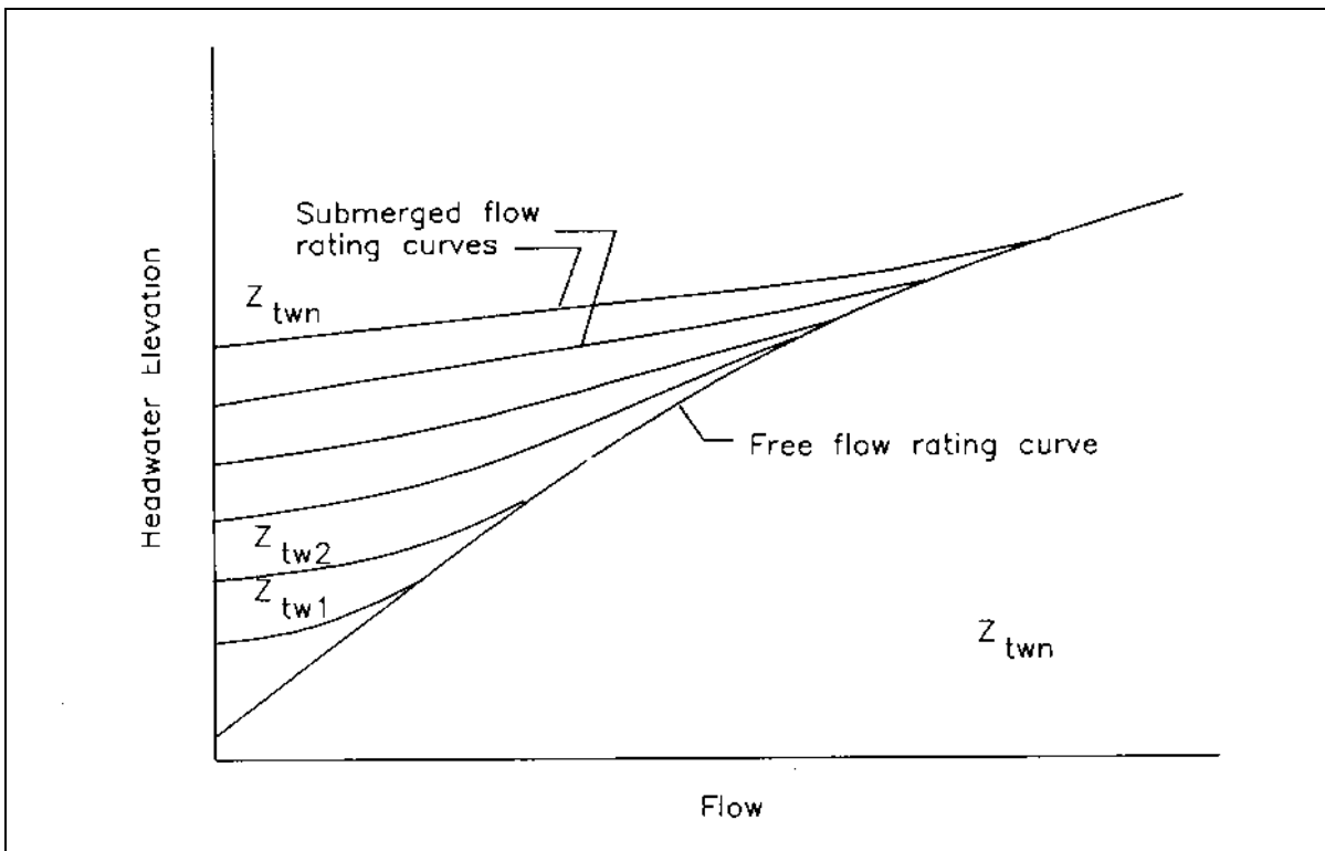
Figure D-4. A free flow rating curve and a set of submerged rating curves
