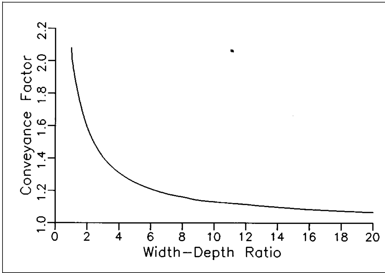
Figure D-3. The relationship between width-depth ratio and the increase in conveyance caused by assuming that the top width is the wetted perimeter for a rectangular channel
