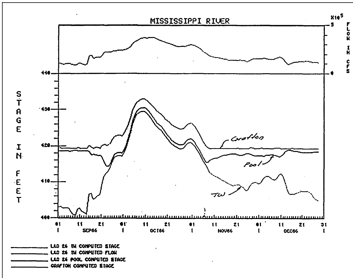
Figure D-6. Pool, tailwater, and control point hydrographs at Lock and Dam 26
