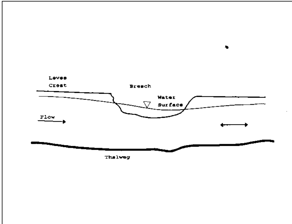
Figure D-11. The water surface of a river at a levee breach
