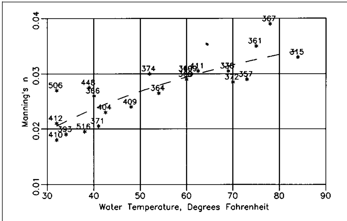
Figure D-15. Plot of Manning's friction factor n against water temperature for Middle Loup River at Dunning, Neb. (Colby and Scott 1965)
