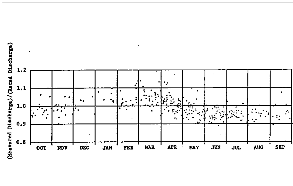
Figure D-19. Seasonal shift shown for the Mississippi River at St. Louis for stages over 20 feet from 1969 to 1983
