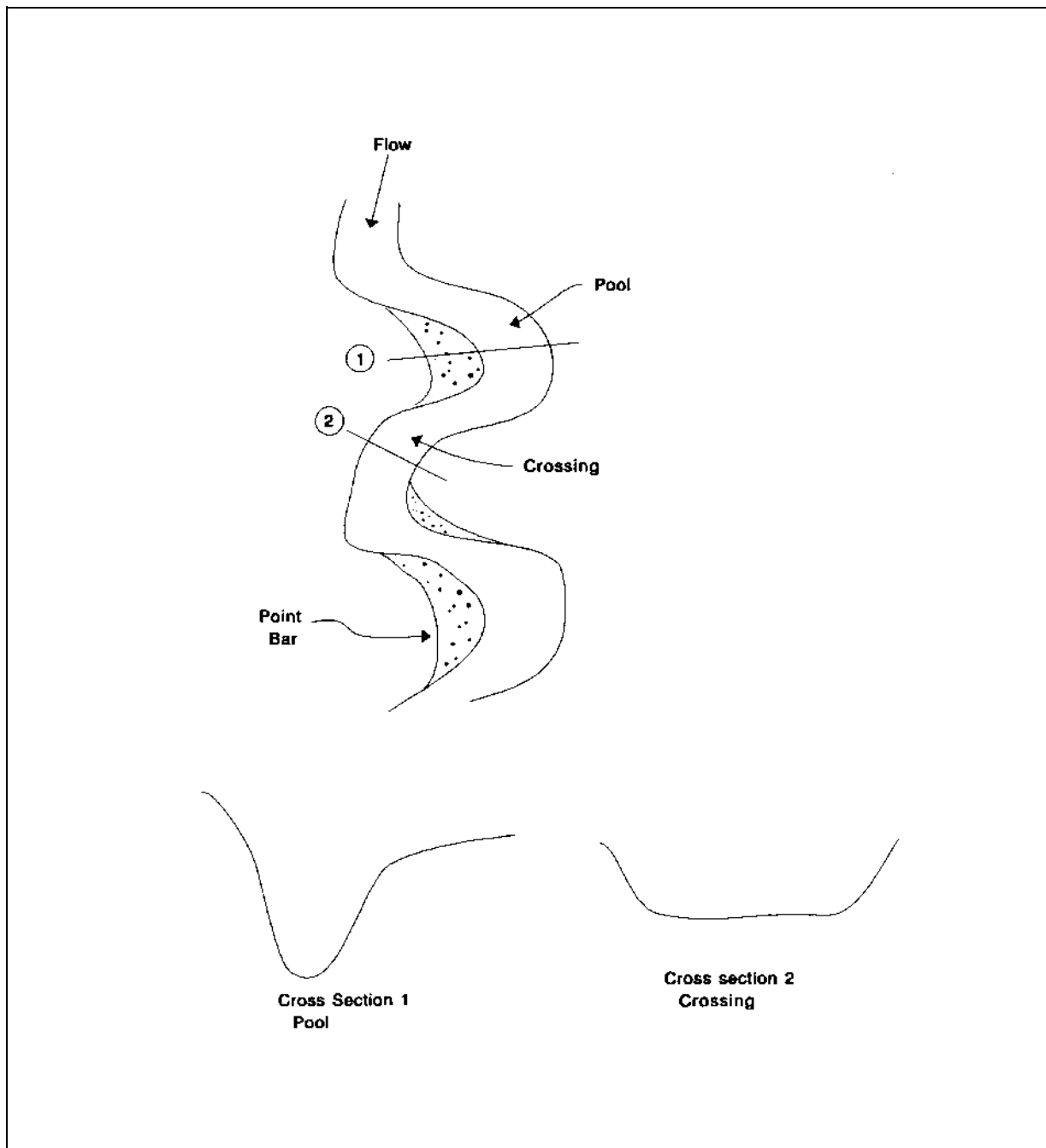
Figure D-1. Pool-riffle sequence in a river
