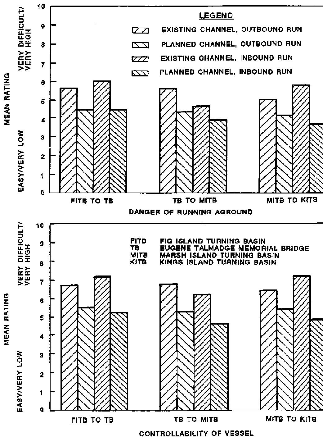
Figure C-14. Typical results from the ship simulator study
