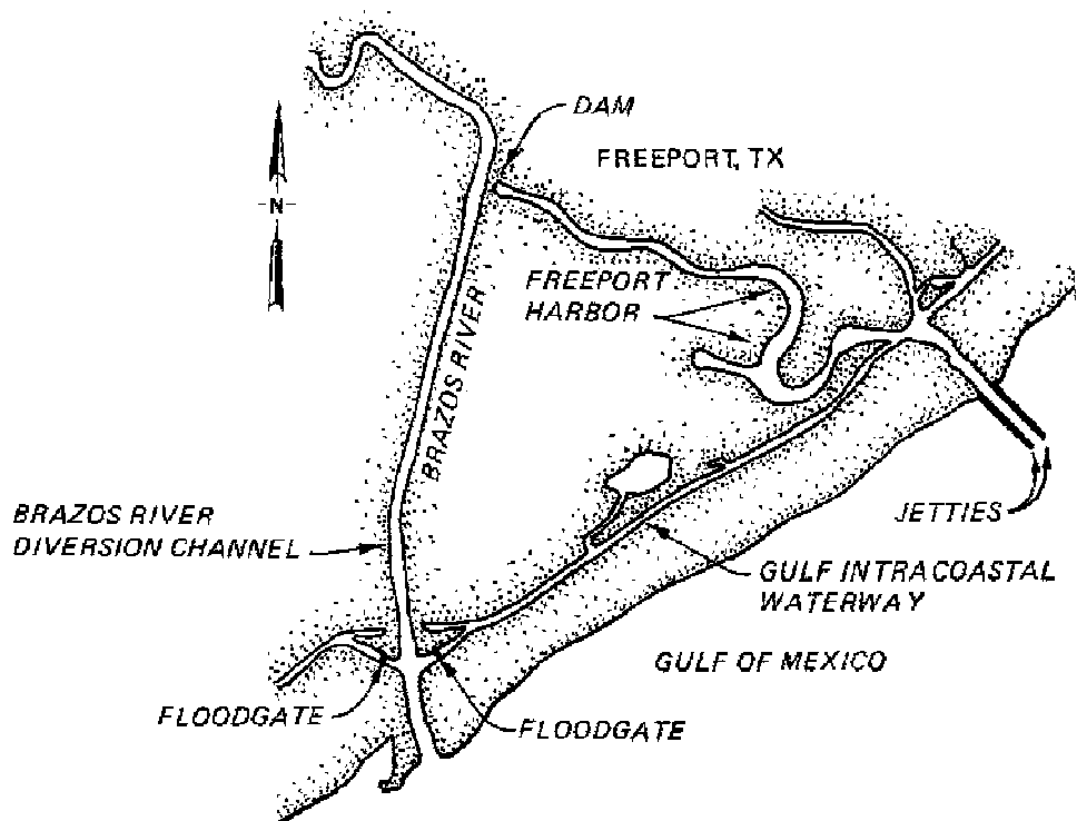
Figure 5-7. Flow diversion
