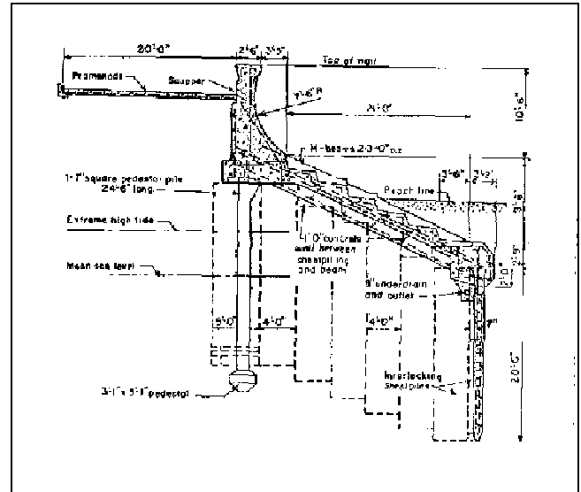
Figure C-6. Combination stepped- and curved-face seawall cross section
