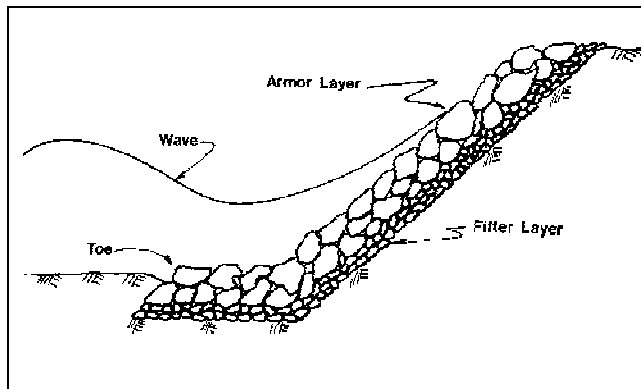
Figure 3-1. Typical revetment section
