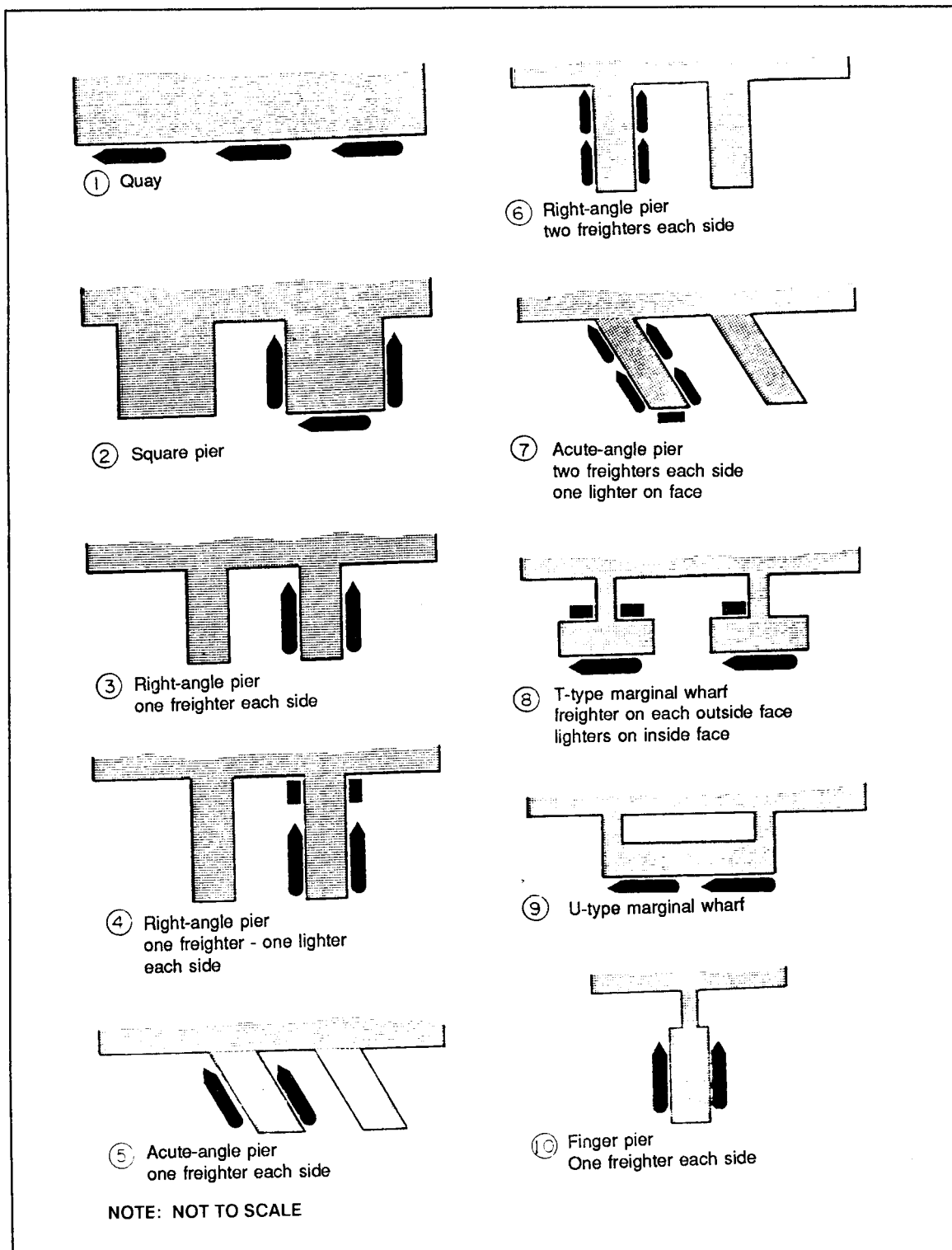
Figure 3-1. Wharf Layout
