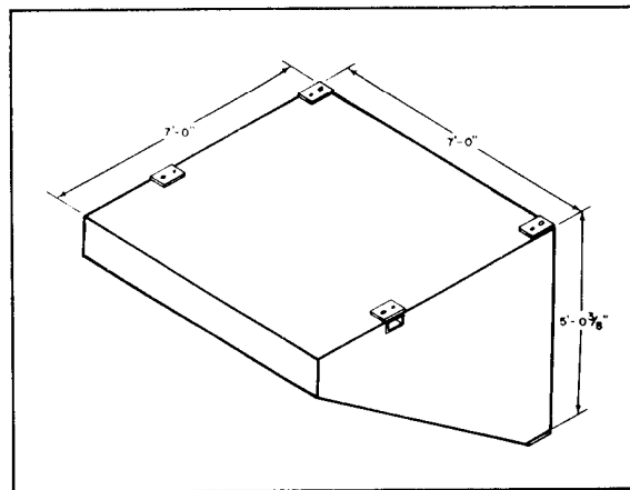
Figure 10-5. P2 Pontoon
