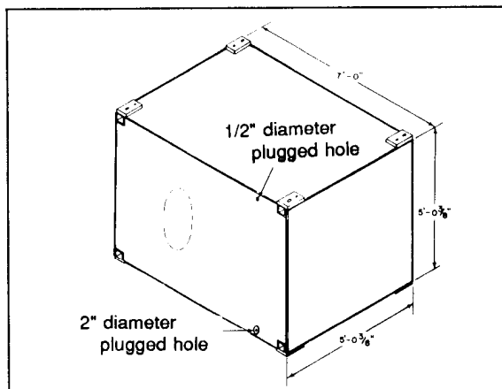
Figure 10-4. P1 Pontoon
