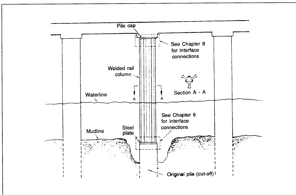
Figure A-9. Welded Steel Rail Column
