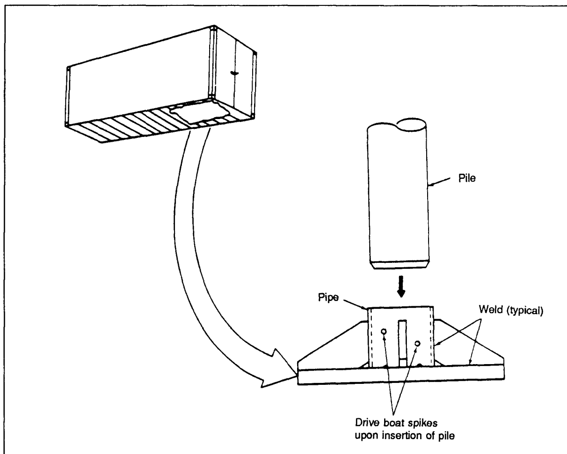
Figure 12-3. Container-Floor or Steel-Plate Foundation
