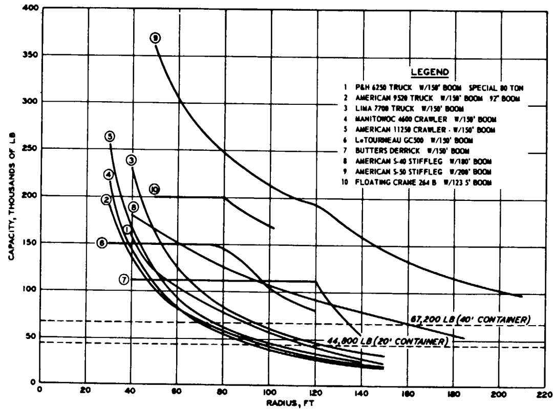
Figure 12-6. Crane capacity.
