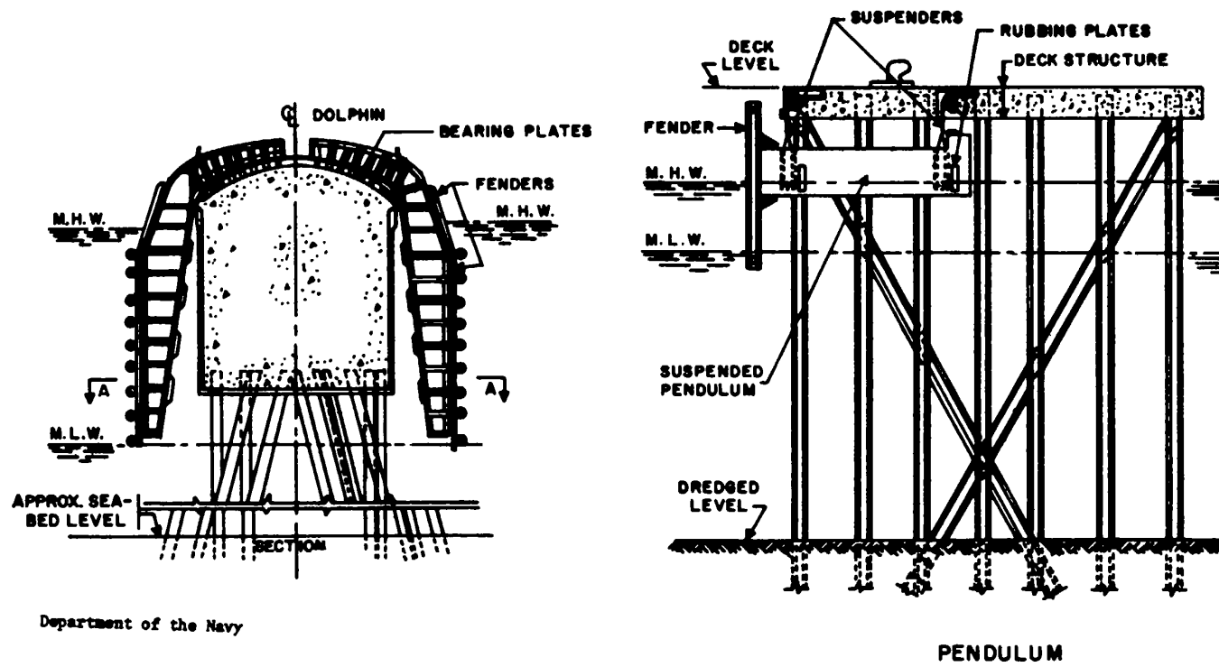
Figure 9-19. Suspended fender. 9-29
