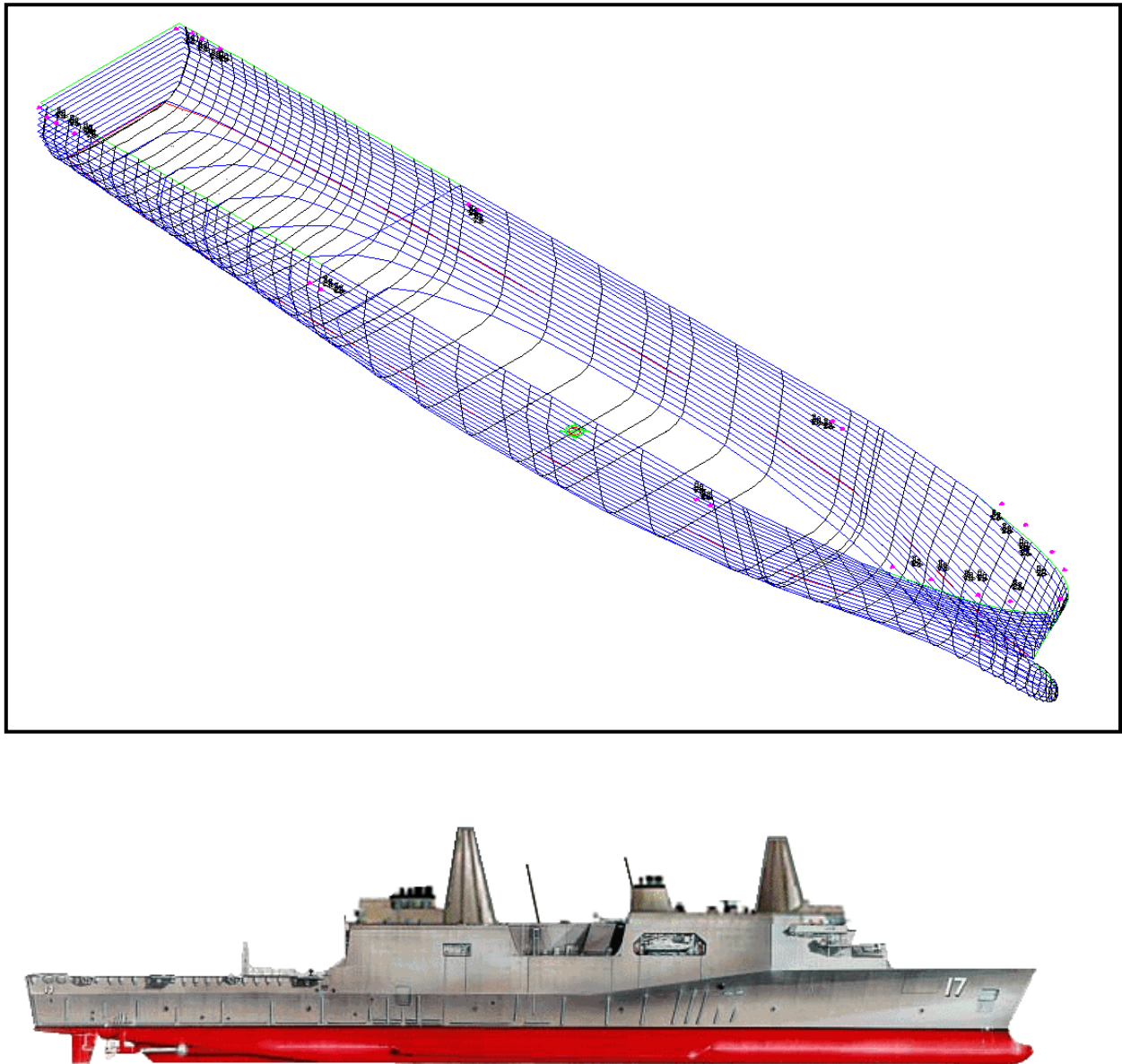
Figure 8-17. LPD-17 USS SAN ANTONIO (Upper – hull form and mooring fitting locations, Lower – profile view)
