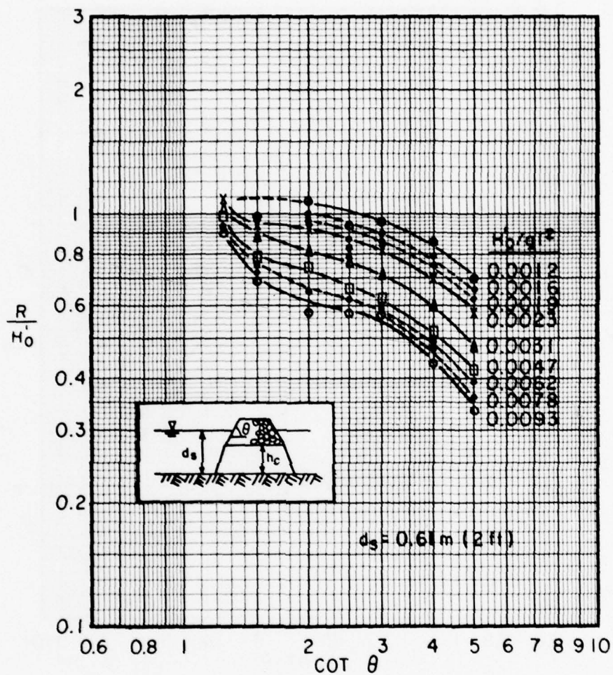
Figure 27. Quarrystone rubble-mound runup; d_s/H_0' = 8.0 ; H_0'/k_p = 1.7 ; h_c/d_s \approx 0.75 (after Hudson, 1958).
