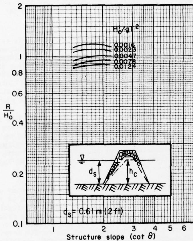
Figure 28. Quarrystone rubble-mound runup ("smooth" stones); random placement; d_s/H_0' = 5.0 ; H_0'/k_p = 2.7 ; h_c/d_s \approx 1.10 (after Jackson, 1968a).
