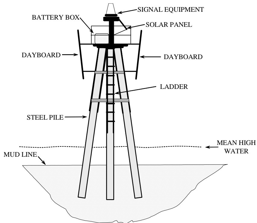
Figure 6-2 - Battered Pile Steel Structure
