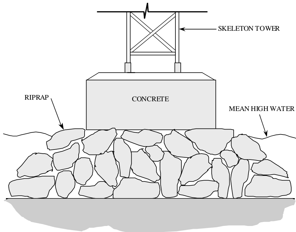
Figure 16-1 - Riprap Foundation
