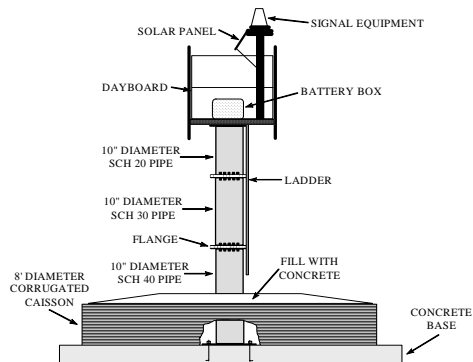
Figure 5-1 - Spindle Structure with Flange Connections
