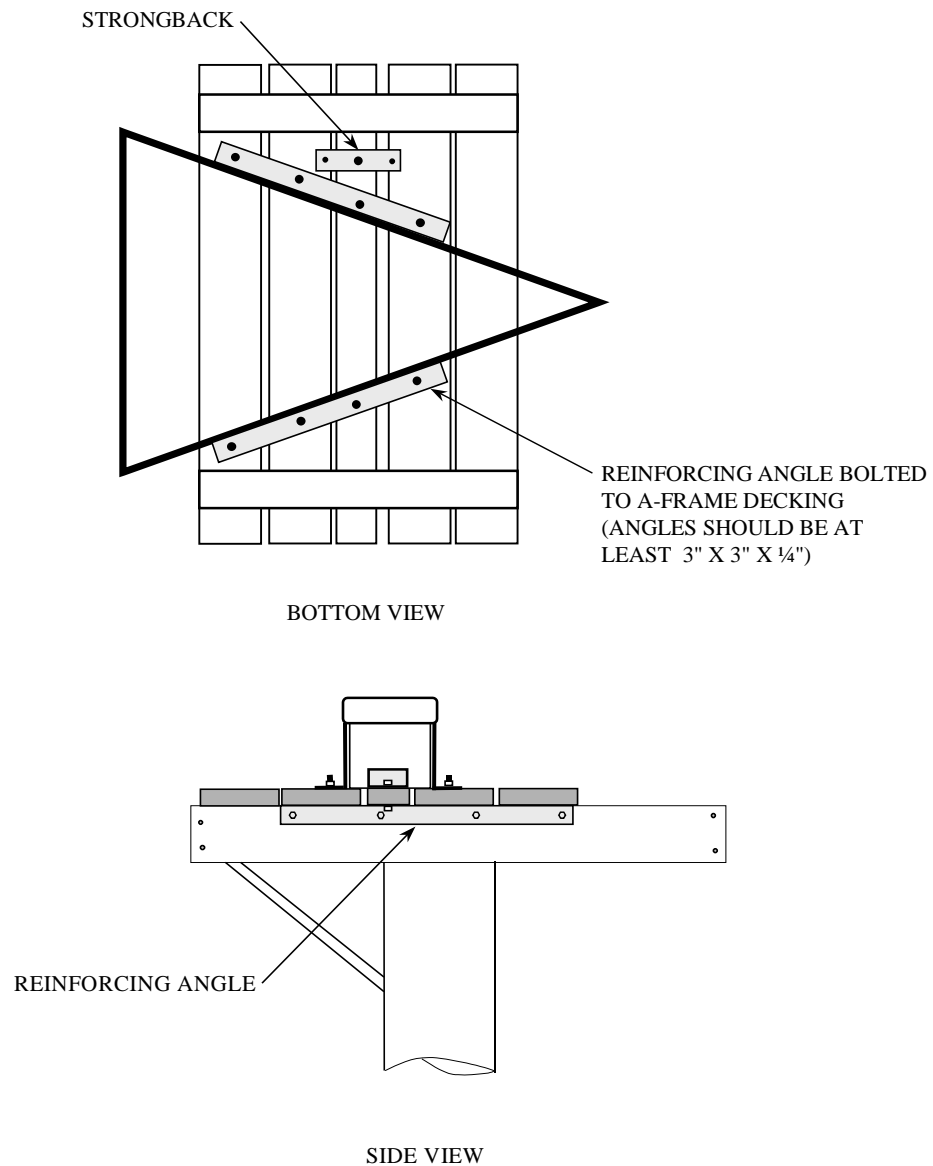
Figure 21-3 - Platform Reinforcement
