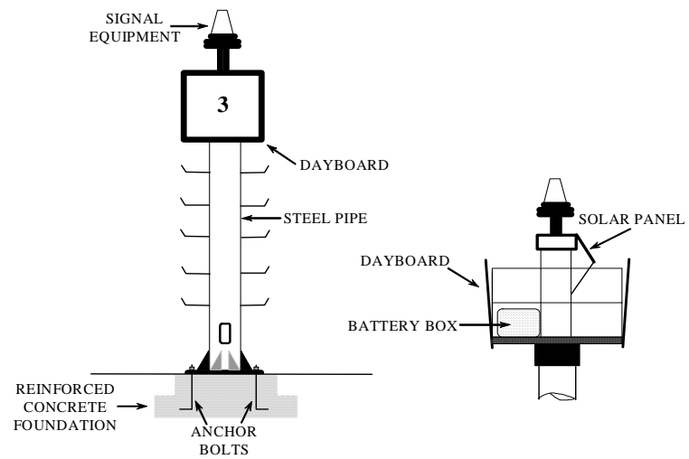
Figure 4-1 - Post Structure
