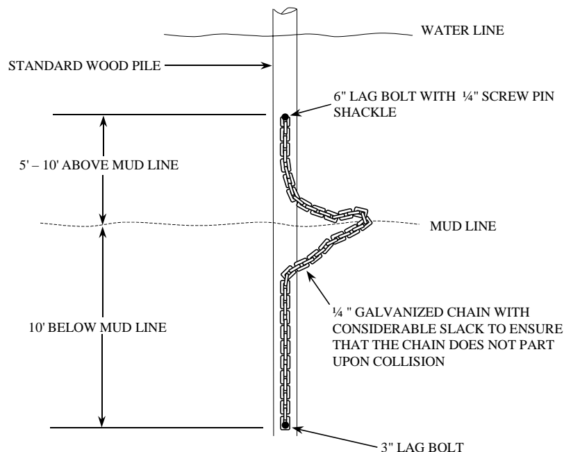
Figure 21-2 - Pile Tethering
