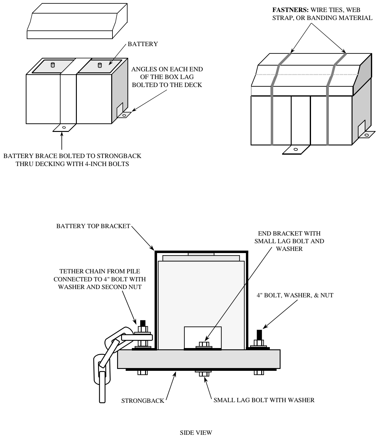
Figure 21-1 - Battery Bracing
