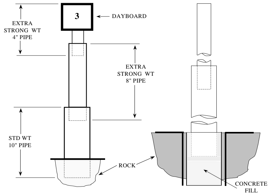
Figure 5-2 - Spindle Structure with Gravity Connections
