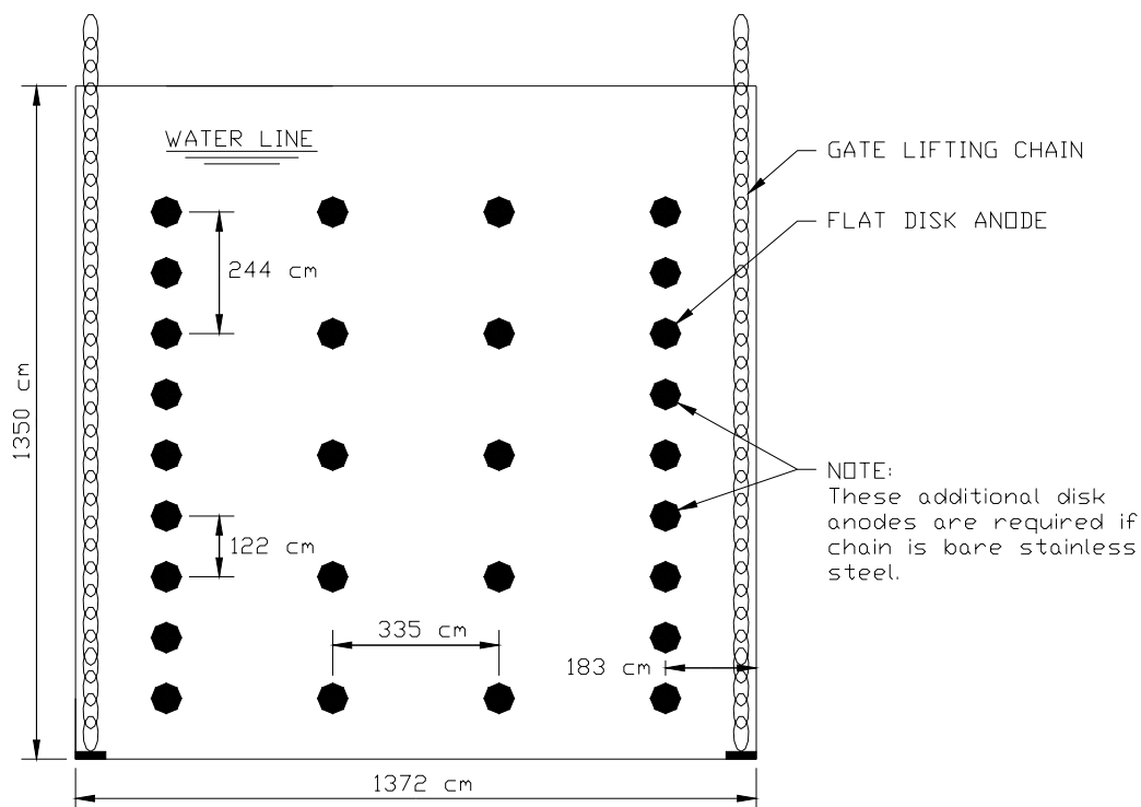
FIGURE B-7. TAITER GATE DESIGN AT CORDELL HULL SHOWING FLAT DISK ANODE PLACEMENT
