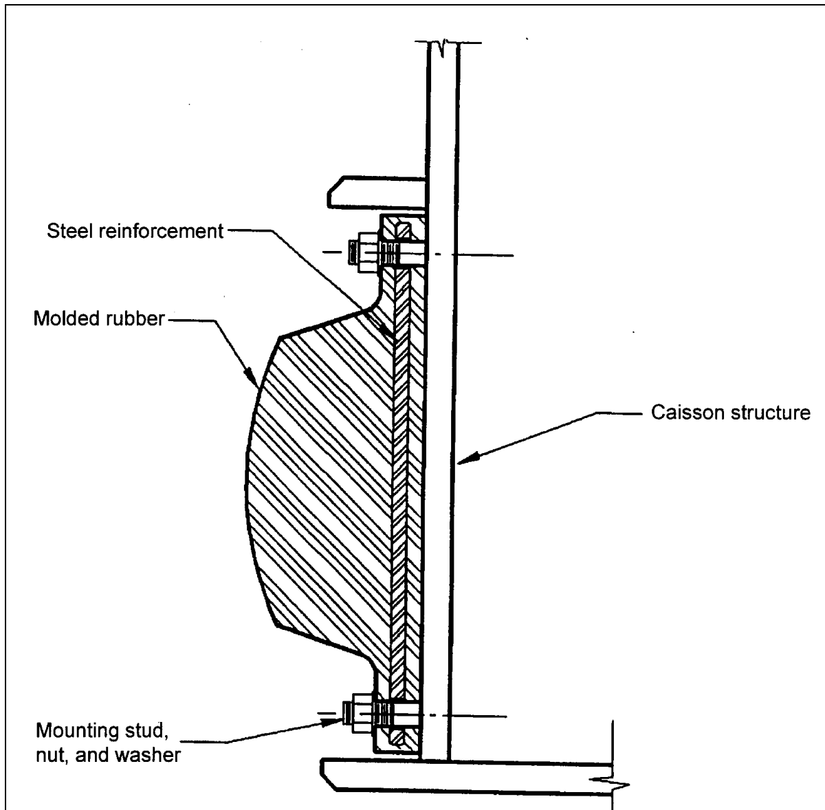
Figure 9-2 Steel Reinforced All-Rubber Caisson Seal Assembly
