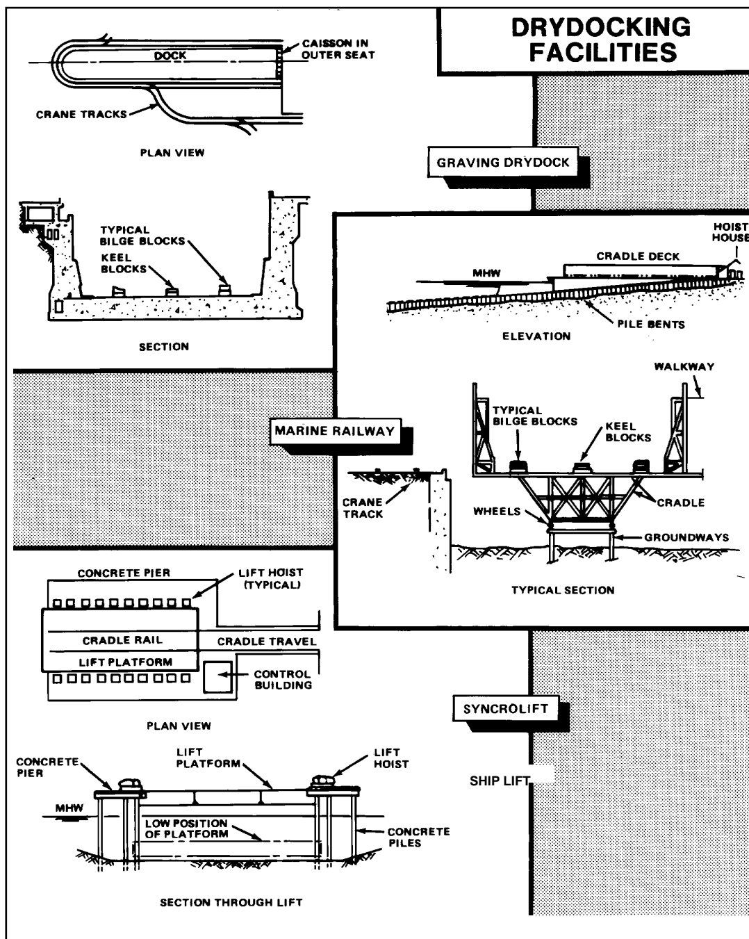
Figure 2-5 Drydocking Facilities
